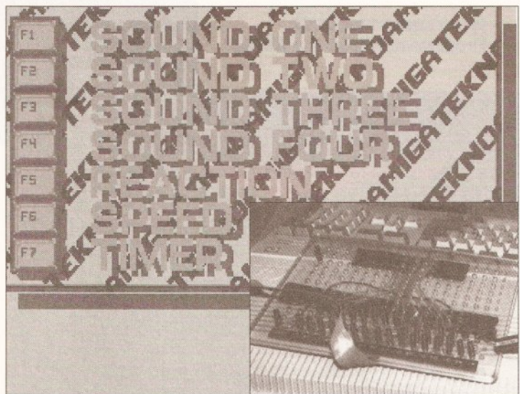
Tekno Amiga - each of the sound menus contains four sampled sounds which can be triggered using the experiment board. (Inset - the perspex experiment board which can be used to mount electronic components)
