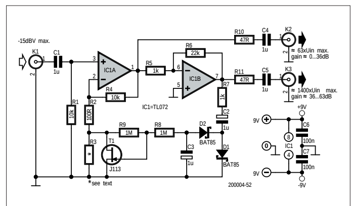
Figure 2: An automatic gain control does not have to be extremely complicated.
