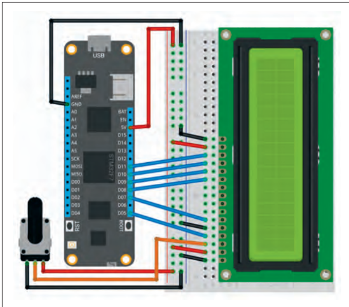
Figure 6: Hook the LCD up on a plug board (Image: Wilderness Labs [5]).
