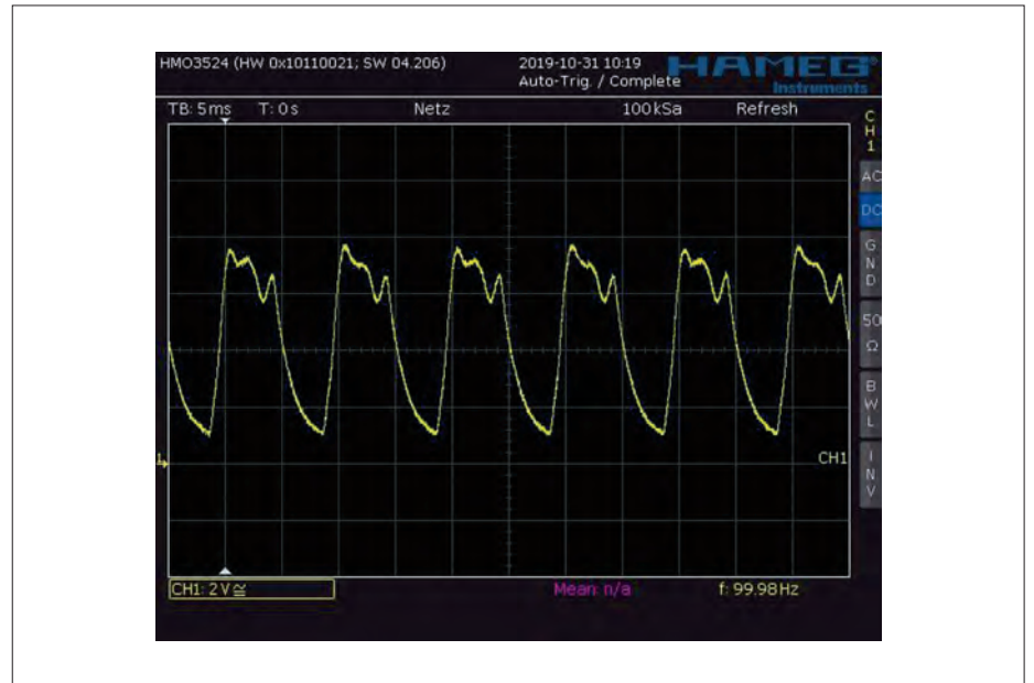
Figure 4: Oscillogram of the 100-Hz ripple of light, superimposed with higher frequency components.
