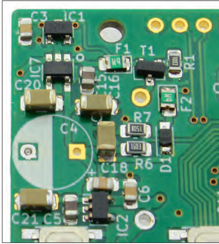
Figure 3. Board space reserved for electrolytic capacitor C4, one of the largest parts on the board.
