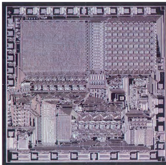
Figure 3. TMS1000 die. Source: State of the Art, by Stan Augarten. http://smithsonianchips.si.edu/augarten/i38.htm
