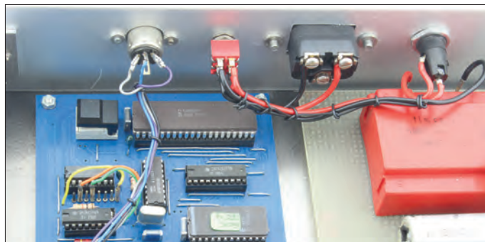
Figure 3: Elements installed on the back panel of the Intelekt case and not normally accessible to the audience. Also note the PCB space reserved for the INT pushbutton which is wired as an external part.
