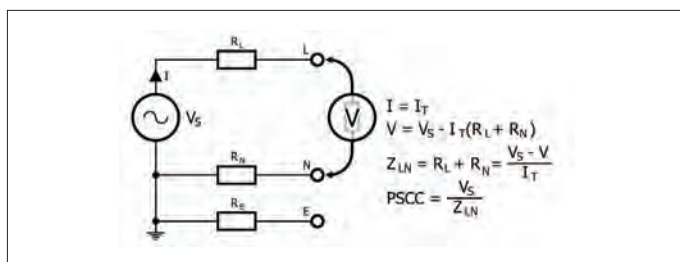
Figure 3: The PSC Tester causes a test current of a known value to flow to calculate the circuit's impedance.
