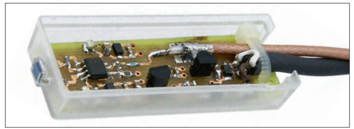
Figure 3: My optical probe with milled circuit board. In the front you can see the photodiode.
