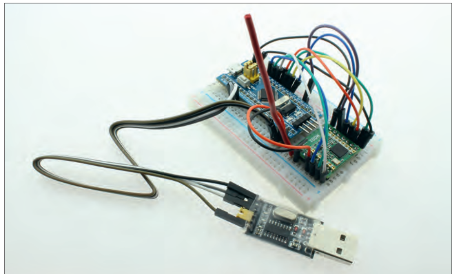
Figure 3. The hardware on the plug-in board with the wired LoRa module.
