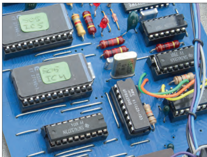
Figure 5: The 8088 has no on-chip clock generator but requires a special IC, the 8284.
