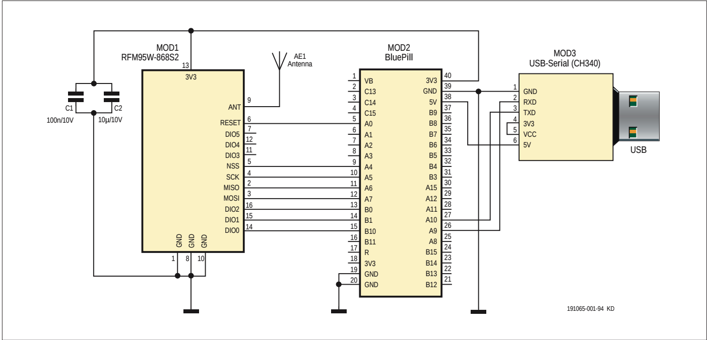
Figure 1. Circuit diagram of the Low-cost LoRa Node.
