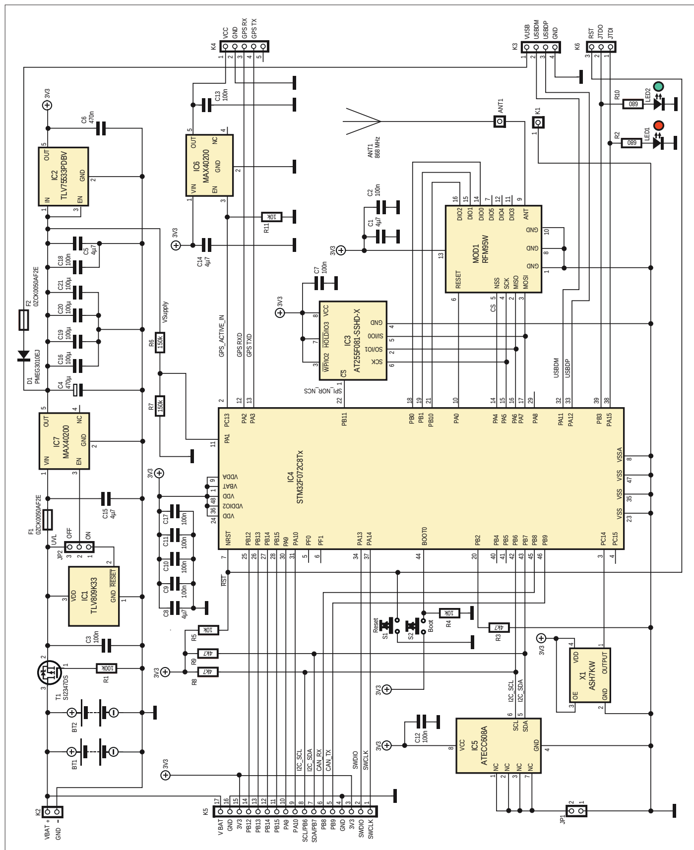
Figure 2. Circuit diagram of the LoRa Node control board. This is basically the LoRaWAN Node Experimental Platform board with a specific outfit of ICs.
