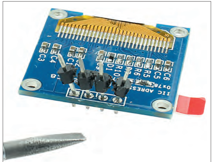
Figure 7. Using a flat screwdriver blade, carefully lever up the plastic remnants surrounding the pins, and remove them.
