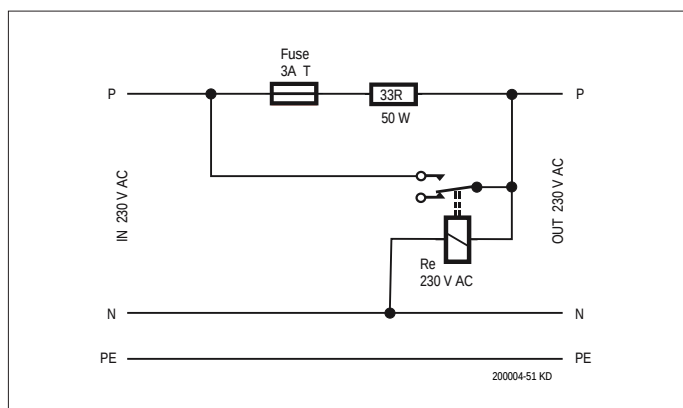
Figure 1: It is hard to make this inrush-current limiter even simpler.
