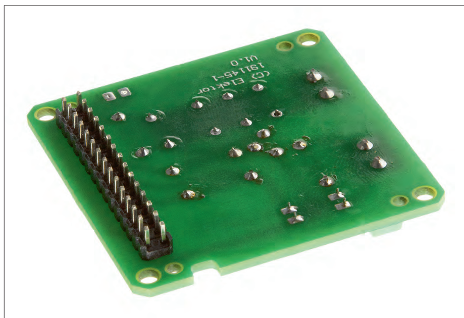
Figure 3: Recommended method of mounting K2: the long pins are inserted from the copper side ('bottom' of the PCB), pushed in upwards, and soldered at the component side.
