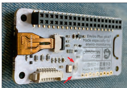
Figure 4. A piece of insulating tape on the bottom of the Enviro+ prevents short circuits.
