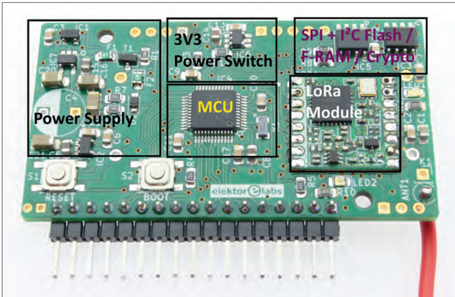
Figure 1. The LoRa Node control board with 'real estate' allocated to functional blocks. Actually, you are looking at a minimally-stuffed LoRaWAN Node Experimental Platform.
