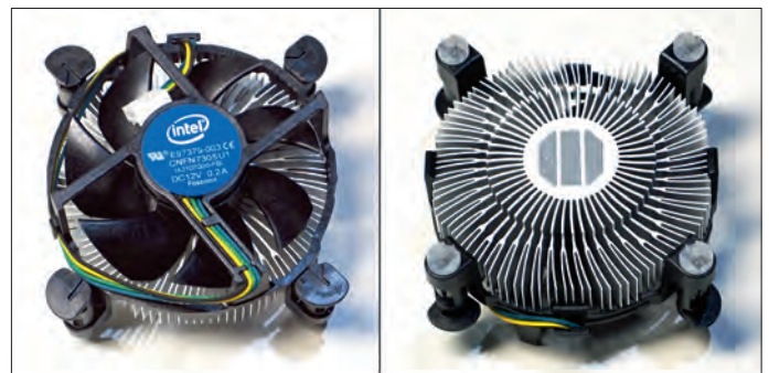
Figure 4: CPU cooler supplied with the 'boxed' version of the processor.
