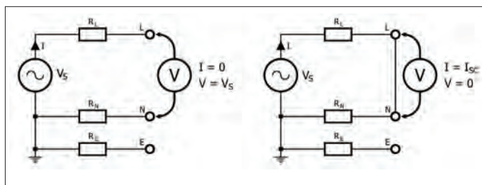
Figure 2: Open-loop voltage measurement (left) & closed-loop short-circuit current (right).
