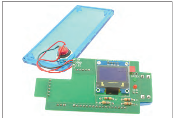
Figure 9. The almost completed LoRa Button board.
