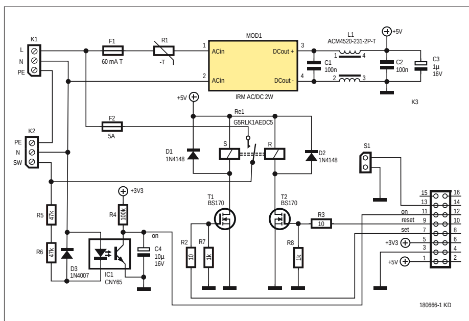
Figure 11. Schematic of the LoRa AC Switch. This is not a ‘dumb’ device but it feeds the actual relay on/off state back to the LoRa Node.
