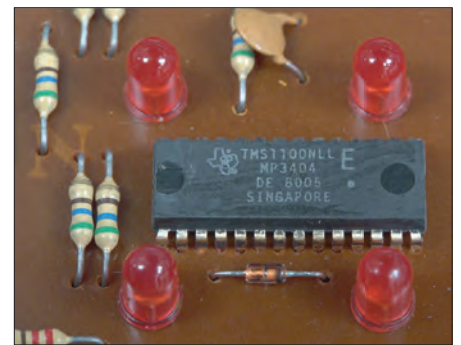
Figure 2. TMS1100 inside a Parker Brothers Merlin Game. Image: 'Binarysequence' - own work, Wikimedia Commons, CC BY-SA 4.0. https://upload.wikimedia.org/wikipedia/commons/a/ad/Tms1100-merlin.png
