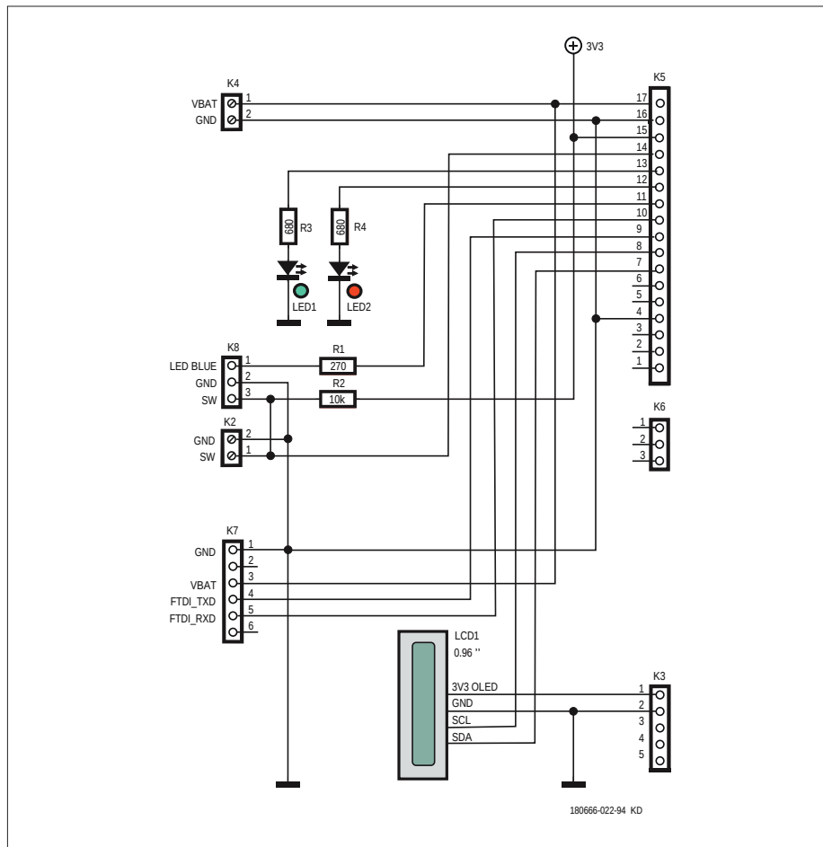
Figure 4. LoRa Button schematic. This is the 'sending' or 'master' part of the Elektor LoRa Node. The OLED display is optional and its use requires deep thought about energy use!
