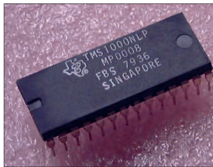
Figure 1. TMS1000 computer on a chip. Image: Christian Bassow, Wikimedia Commons, CC BY-SA 4.0. https://upload.wikimedia.org/wikipedia/commons/d/d1/TI_TMS1000NP_1.jpg
