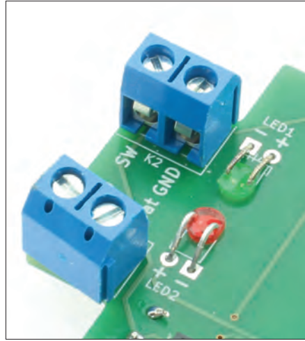
Figure 5. A special method for mounting the LEDs is applied on the LoRa Button board.
