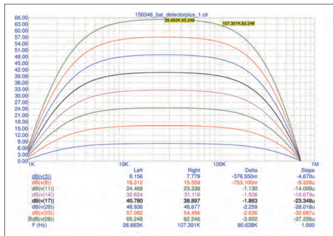
Figure 2: The graph shows the effect of eight identical amplifiers in series (source = 0 \Omega ).
