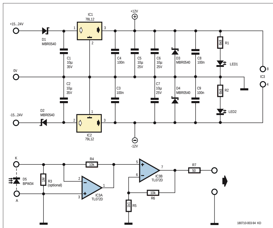
Figure 1: Circuit diagram of the optical probe.
