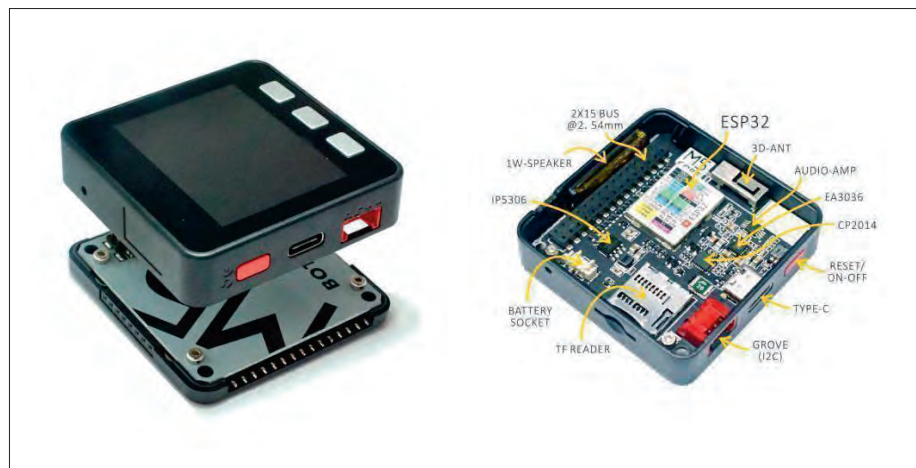
Figure 1: The M5Stack ESP32 Basic Core module available from the Elektor Store.
