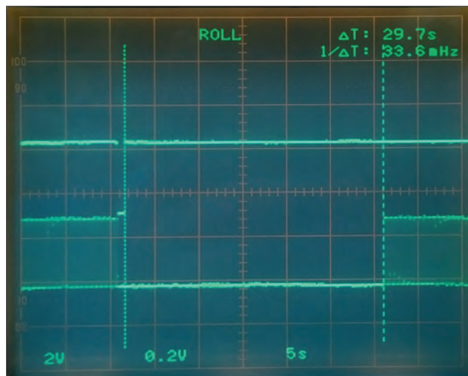
Figure 5: After a reset (upper trace) it takes almost 30 s to get going again.
