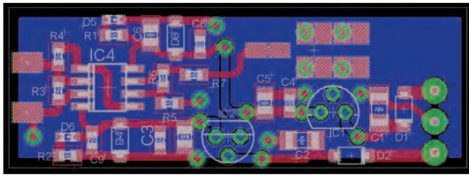
Figure 2: The layout of the scanner board including power supply.
