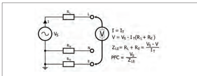
Figure 4: Calculating the prospective earth fault impedance Z_S (or Z_E ) or the Earth fault current P(E)FC.
