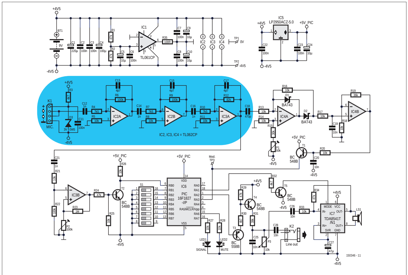
Figure 1: Full circuit of the Bat Detector PLUS with the 3-stage microphone preamplifier highlighted.
