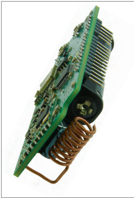
Figure 10. The feedpoint of the home-wound, quarter-wave antenna for the 868-MHz band is soldered to the ANT pad on the LoRa Button board (early prototype shown). Note the coiled construction of the antenna.
