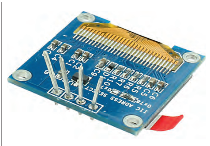
Figure 8. You now have a 'naked' pin row.
