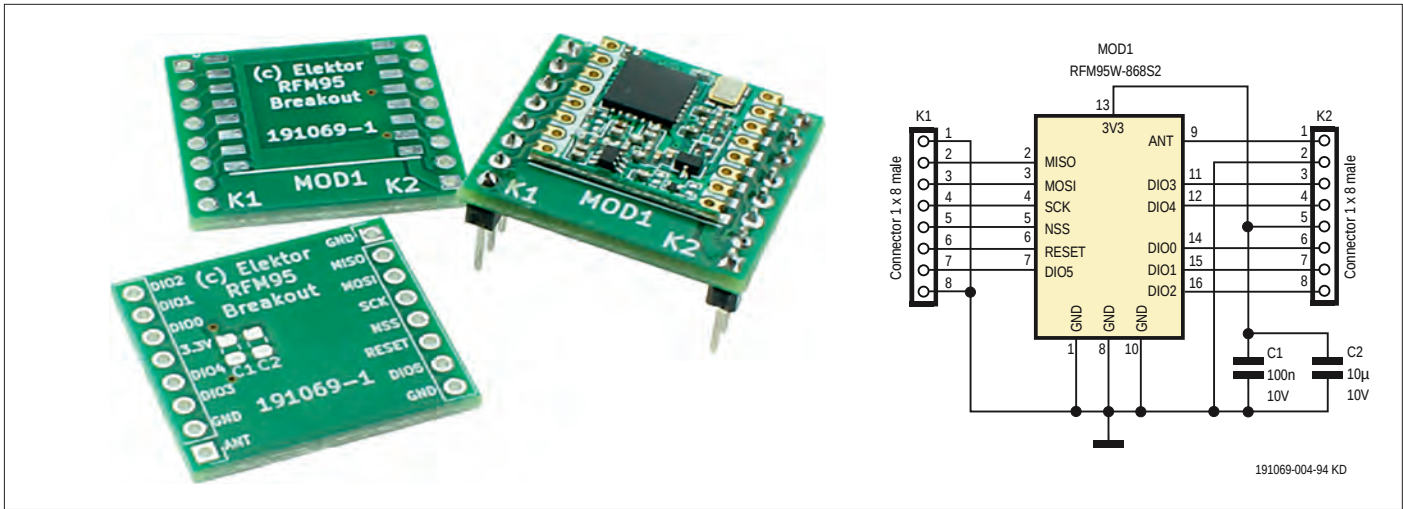
Figure 2. breakout board for the LoRa module.
