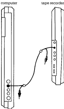
Connect EAR to EAR Connect MIC to MIC
