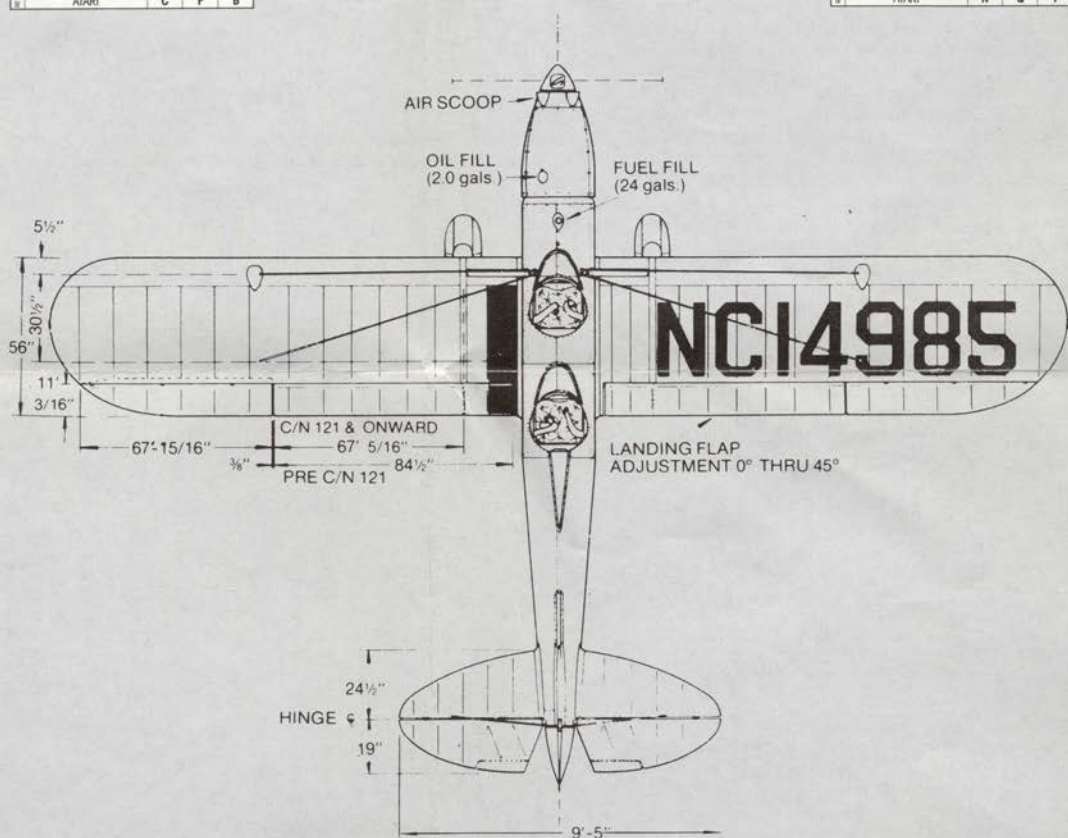
RYAN ST-A (Top View) circa 1934
