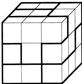
The Soma Cube
