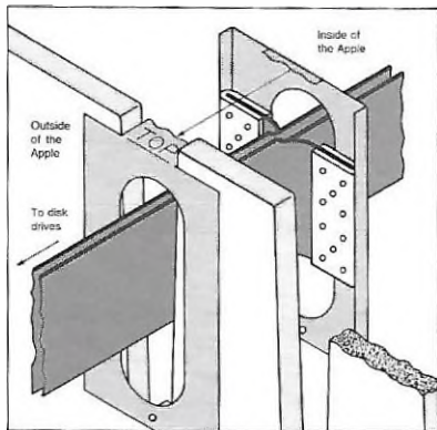
Figure 3-4. Position Two Cables in the Clamp
