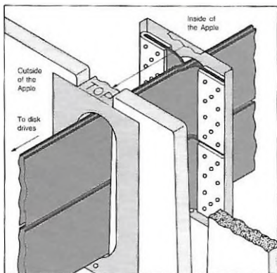
Figure 3-5. Position Four Cables in the Clamp
