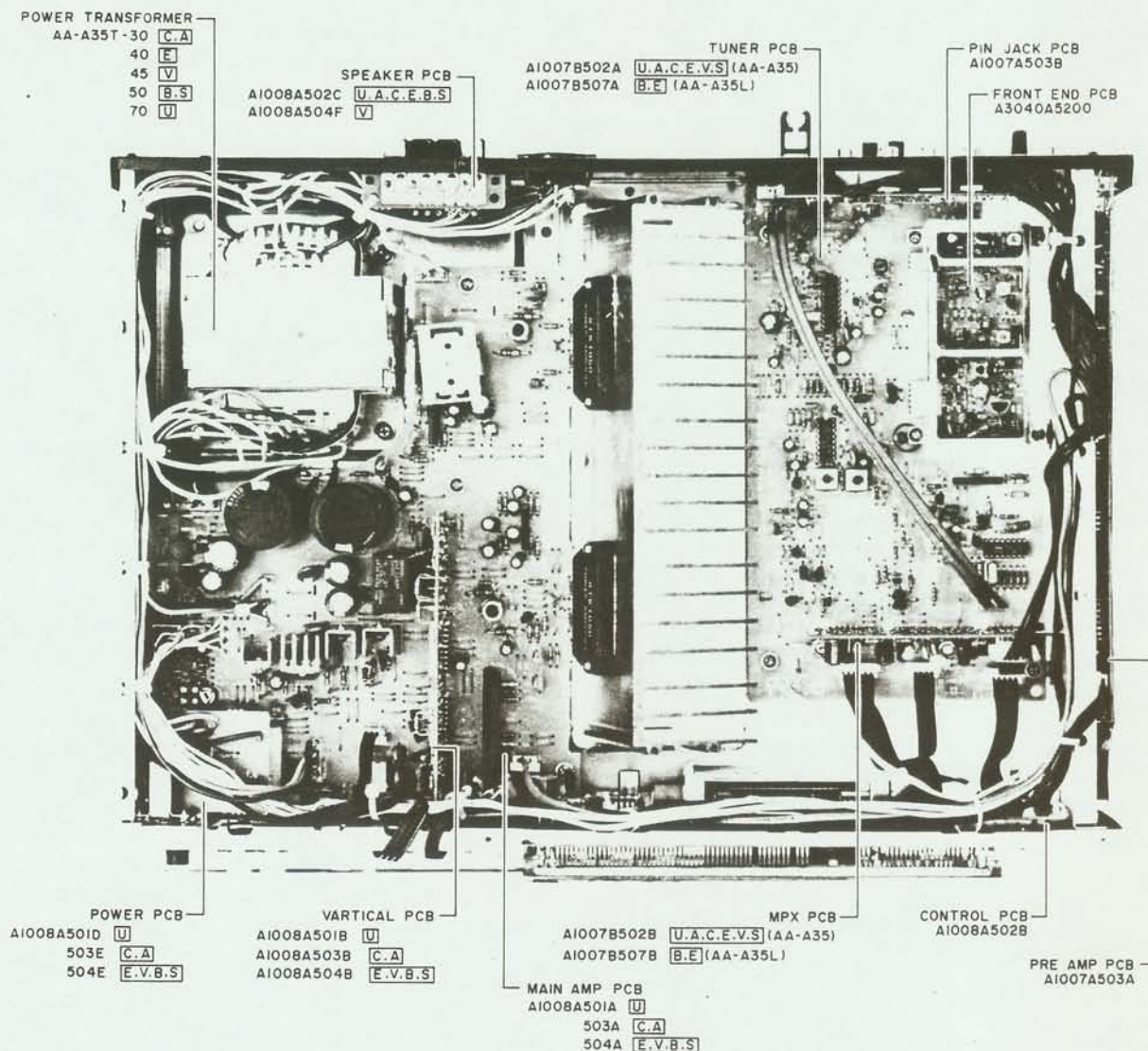
Fig. 4-2 Top View
