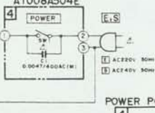
POWER PCB A1008A504E
