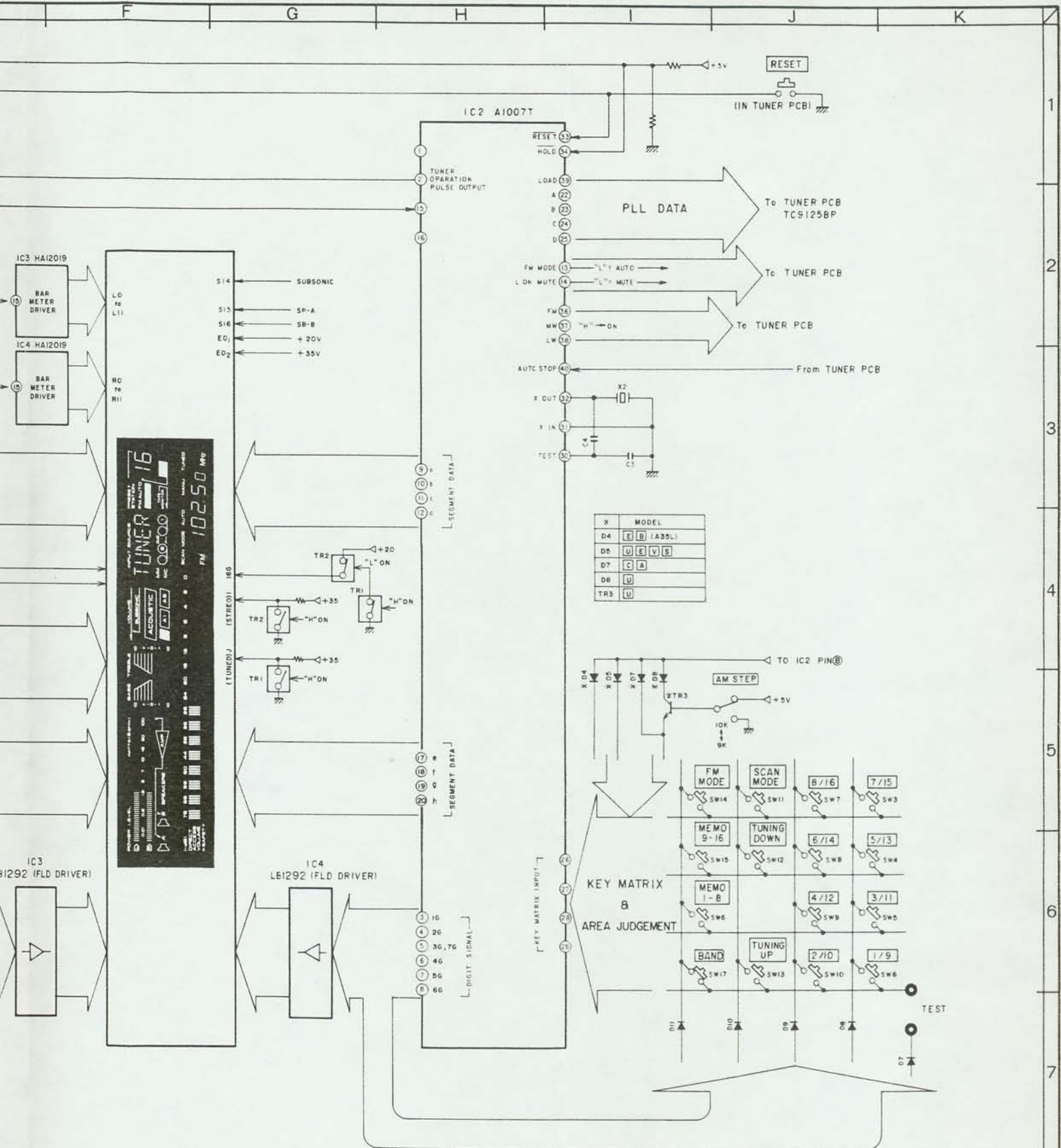
AA-A35/L CONTROL BLOCK DIAGRAM NO.2-1 840601A
