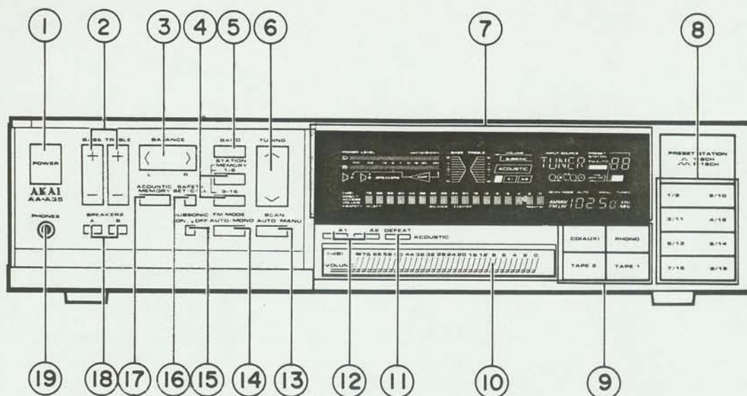
Fig. 3-1 Front View
