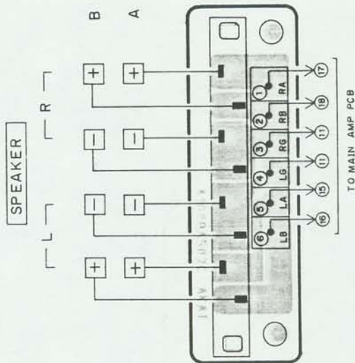
SPEAKER PCB A1008A502C U C A E B S
