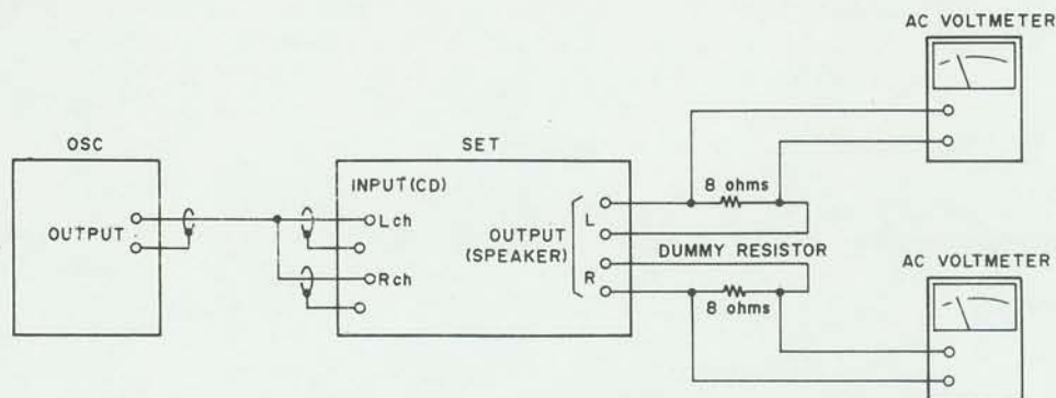
Fig. 6-1 Instrument Connections for Amplifier Section Adjustment
