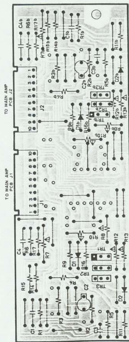
VERTICAL PCB
