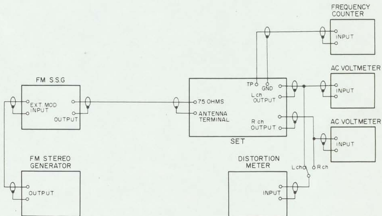
Fig. 7-2 Instrument Connections for FM Section Adjustment
