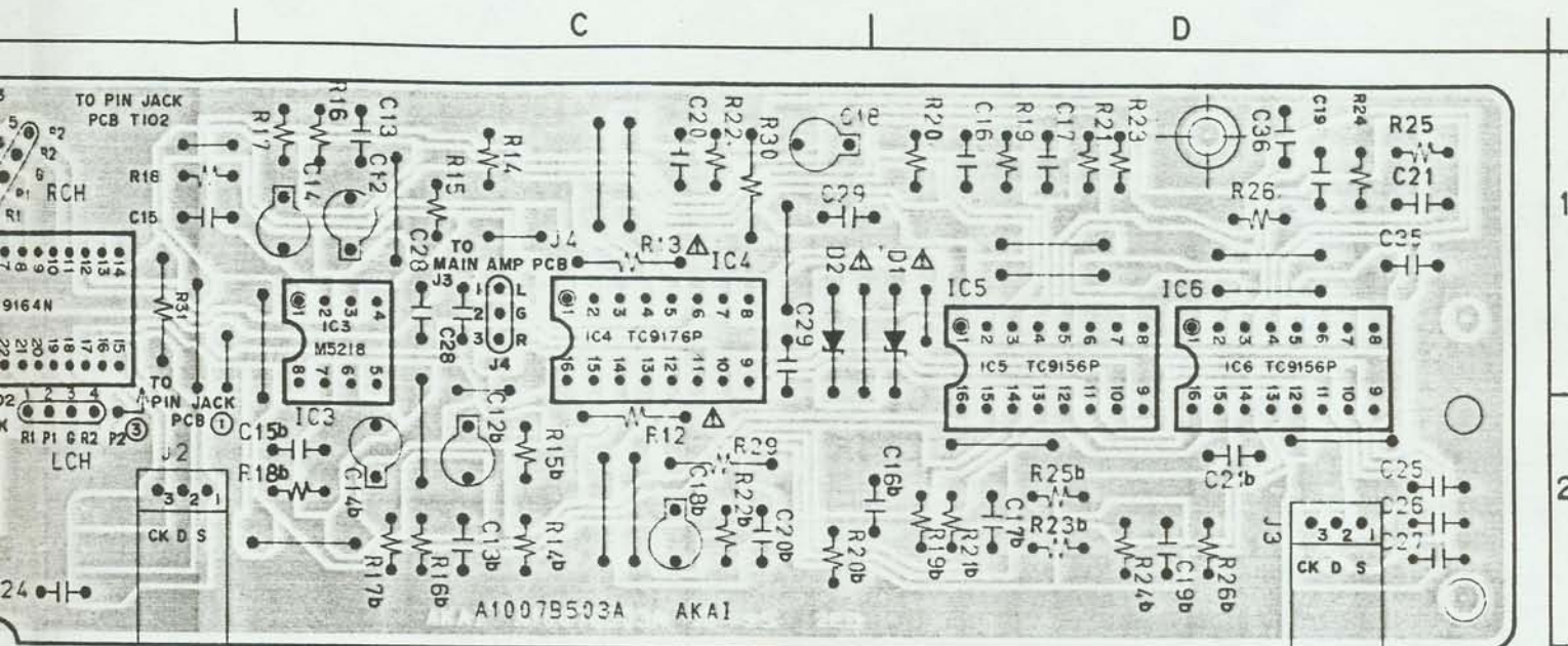
PRE AMP PCB A1007B503A
