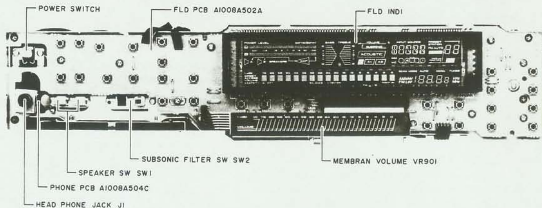
Fig. 4-1 Front View
