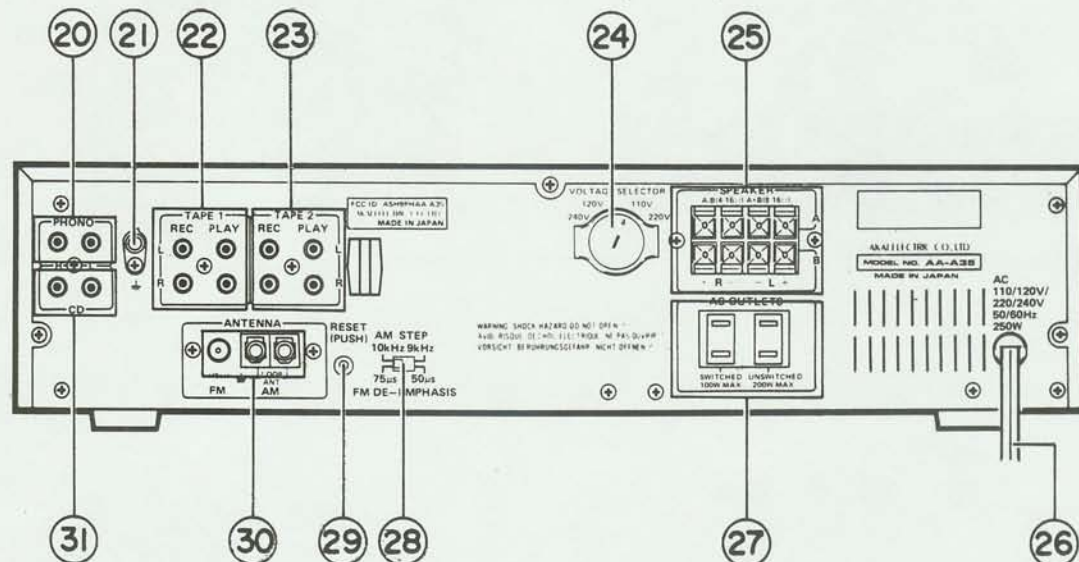
Fig. 3-2 Rear View
