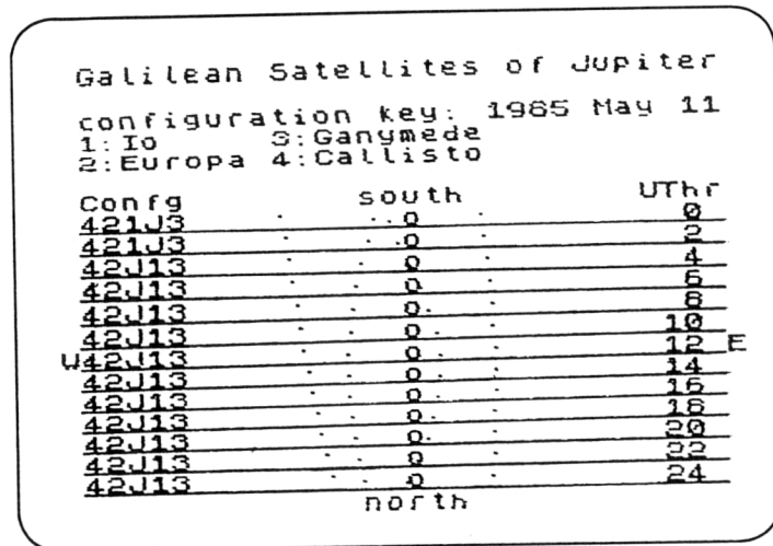
Figure 6.5 The positions of Jupiter's moons for one selected day at 2-hour intervals.
