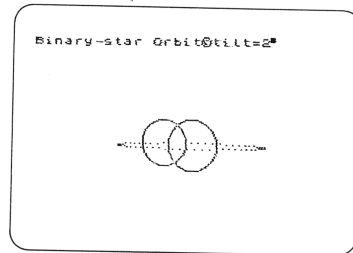
Figure 7.4 Mutual eclipses occur at low angles of orbital tilt.
