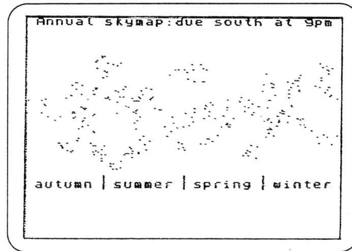
Figure 8.3 A complete starmap of 30 constellations and 310 stars. Ursa Major (the Plough) is top centre and Square of Pegasus extreme left.
