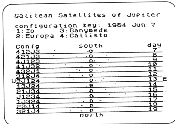
Figure 6.6 This plots the moons at midnight for a 12-day period. The daily motion of the moons is much more pronounced.
