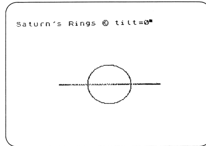
Figure 6.8 Saturn with rings edge-on.
