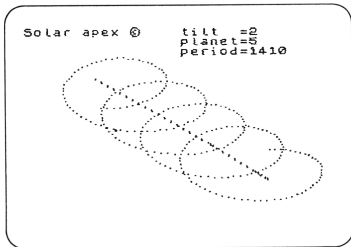
Figure 5.13 Helical motion of a planet through space.
