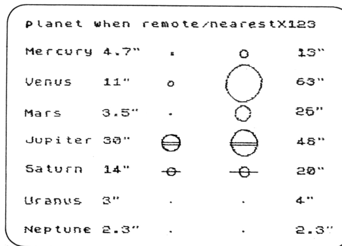
Figure 6.10 Relative size of all the planets in a telescope magnifying \times 123 .
