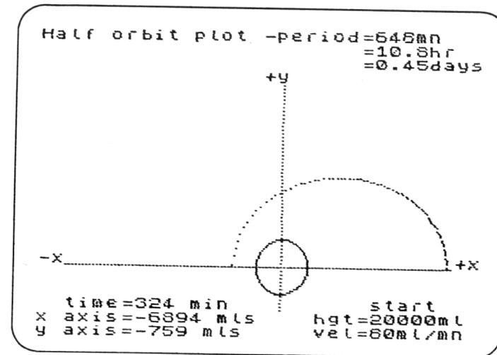
Figure 4.2 Typical orbit plotted from apogee (point adjacent +x sign).
