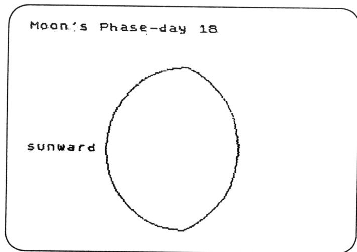
Figure 3.2 Gibbous Moon after 'Full'.
