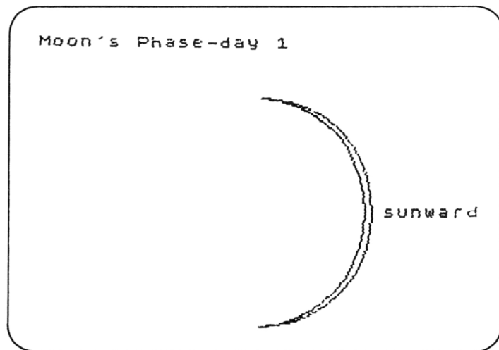
Figure 3.1 The Moon one day old.
