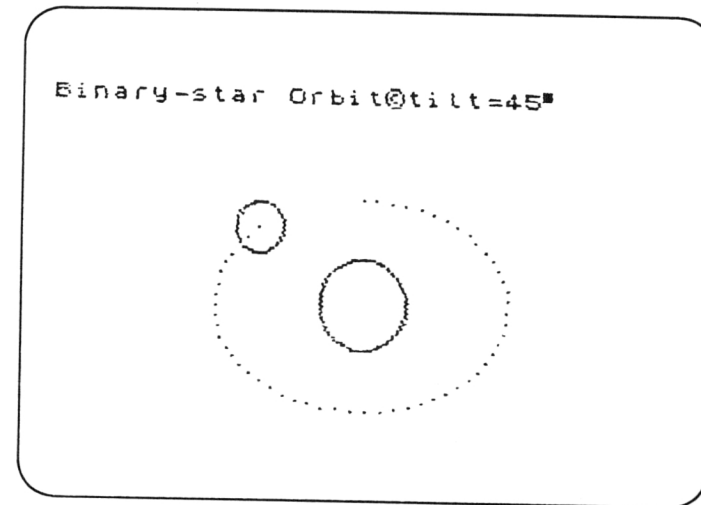
Figure 7.3 A single companion star orbits a massive primary star.
