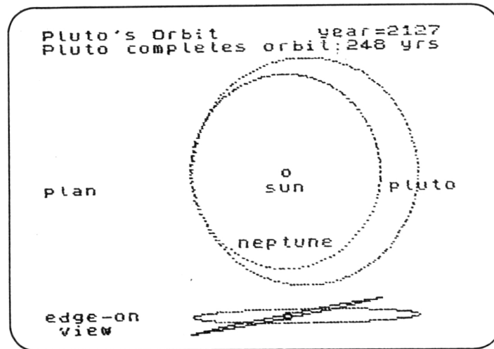
Figure 5.12 The orbits of Pluto and Neptune from two viewpoints.
