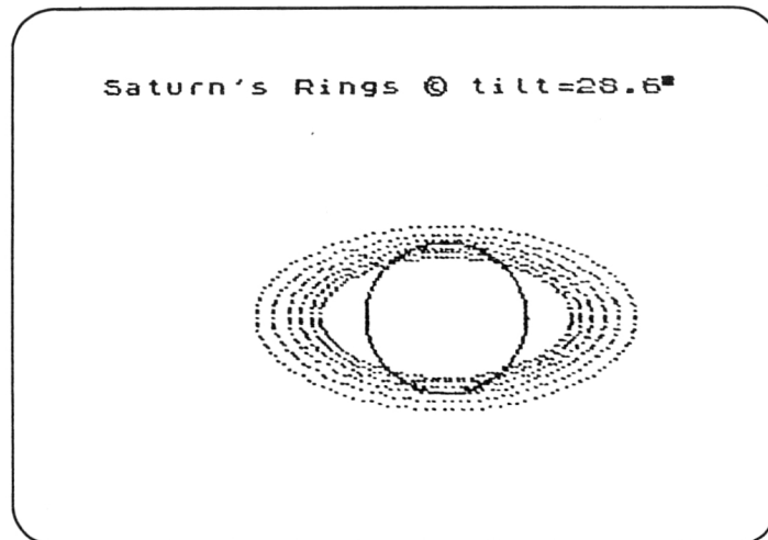
Figure 6.7 Saturn with rings wide open.
