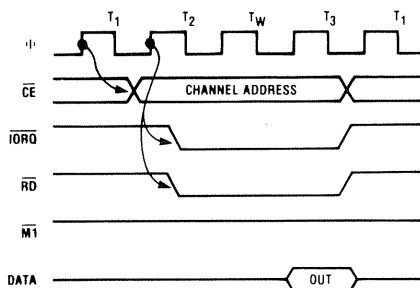
FIG. 14a — READ CYCLE
