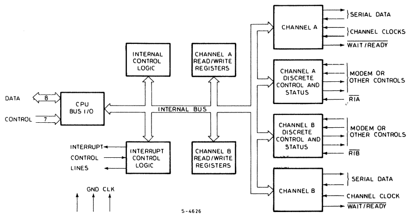
Fig. 3 - BLOCK DIAGRAM
