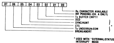
FIG. 12 — READ REGISTER BIT FUNCTIONS
