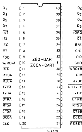
Fig. 2 - PIN ASSIGNMENTS
