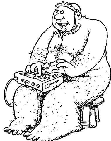
Regression analysis.
