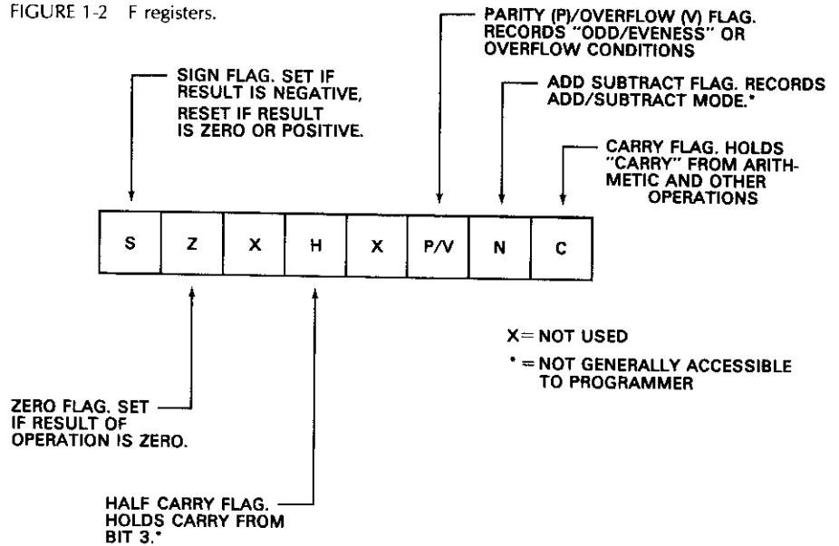
FIGURE 1-2 F registers.
