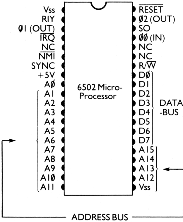
Fig. 10.1: The 6502 Micro-Processor
