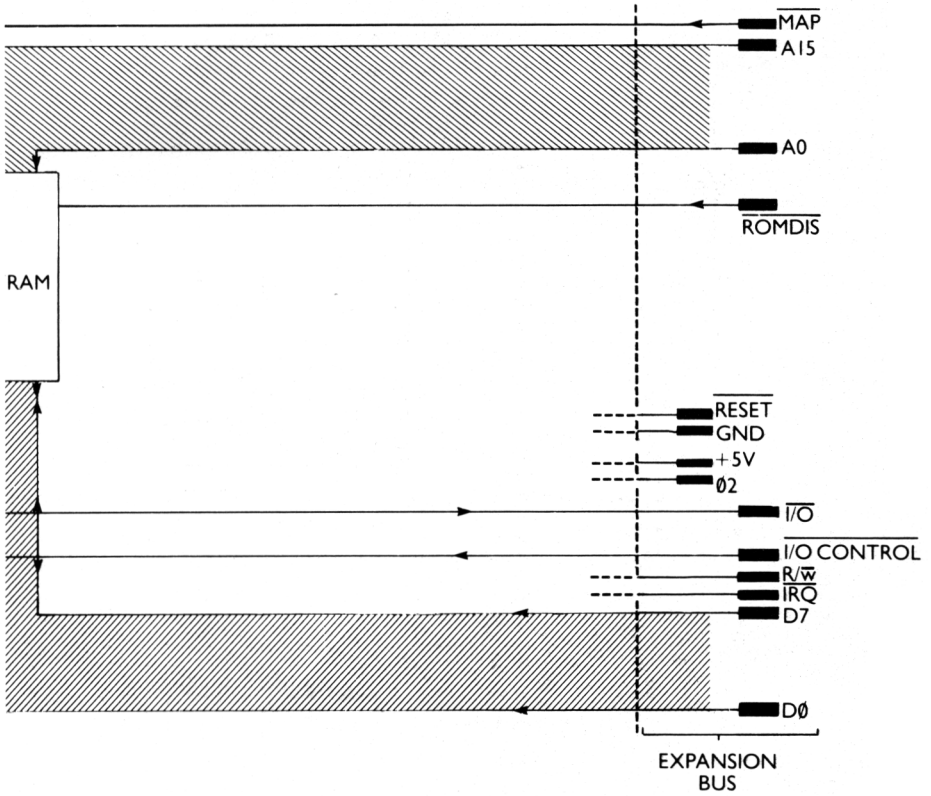
ORIC-1 BLOCK DIAGRAM SHOWING EXPANSION BUS PIN-OUT
