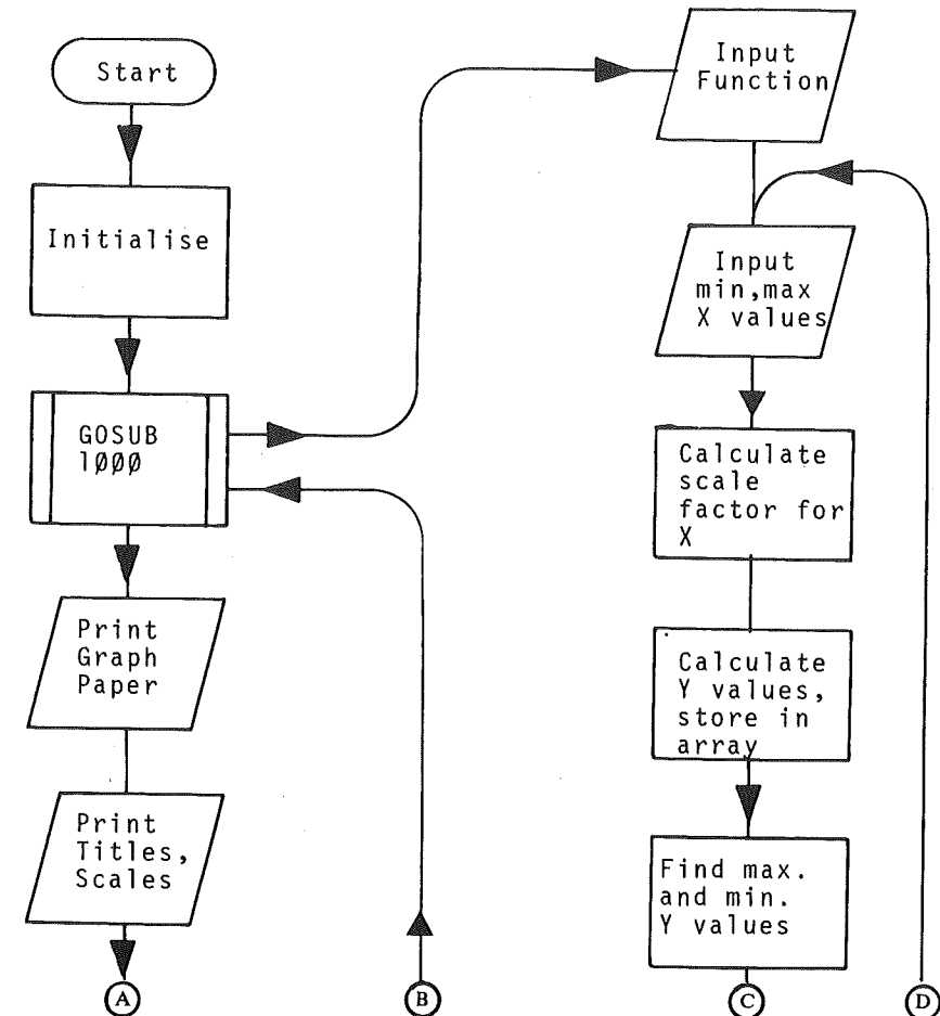
Flowchart "GRAPH"
