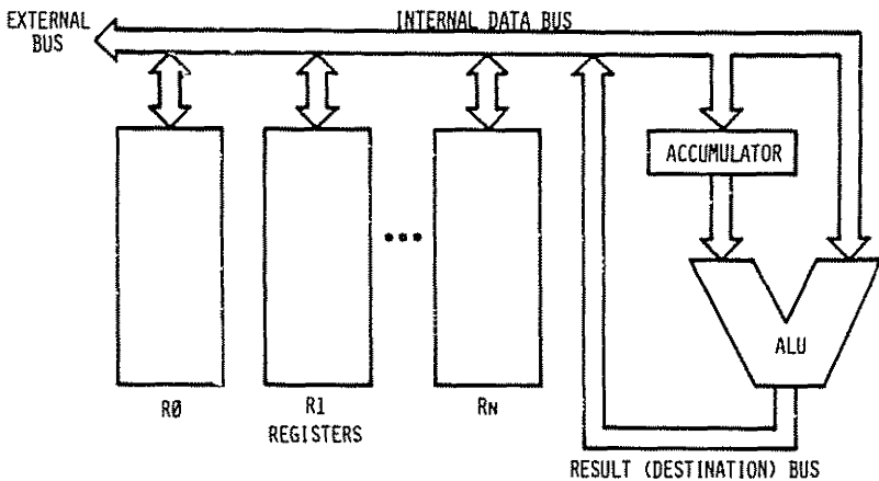
Fig. 2.8: Single-Bus Architecture
