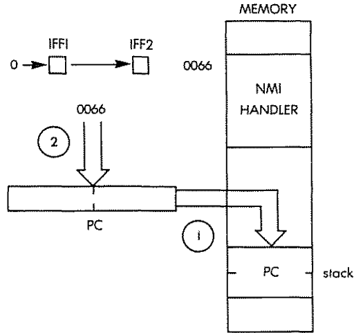
Fig. 6.25: NMI Forces Automatic Vectoring
