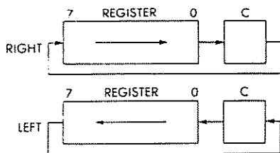
Fig. 4.11: Nine-Bit Rotation
