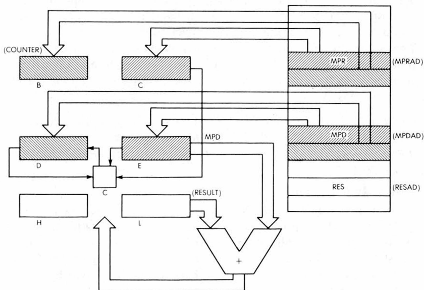
Fig 3.14: 8 × 8 Multiplication—The Registers
