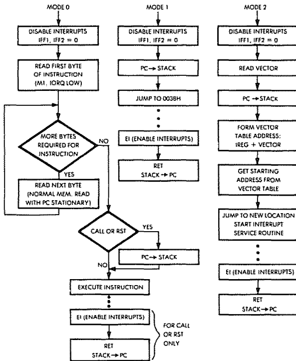
Fig. 6.26: Interrupt Modes
