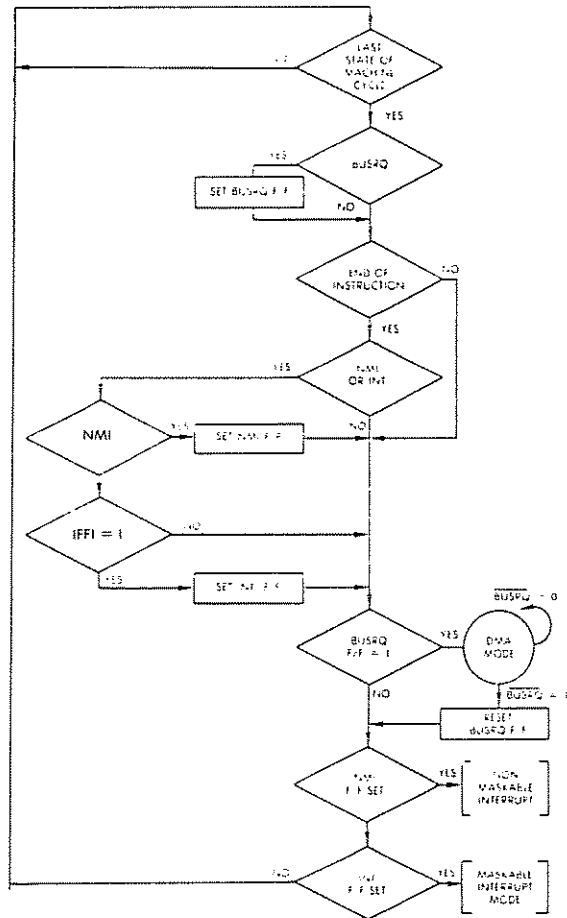
Fig. 6.24: Interrupt Sequence
