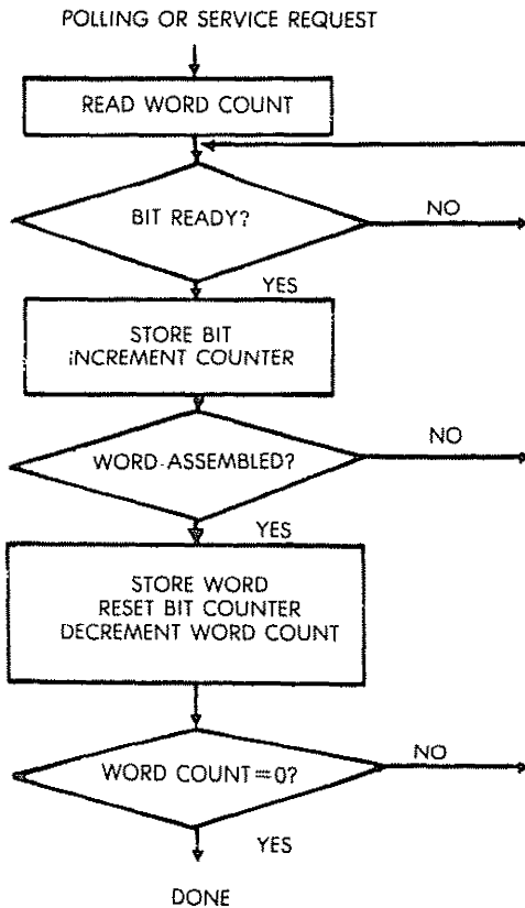
Fig. 6.6: Bit Serial Transfer—Flowchart
