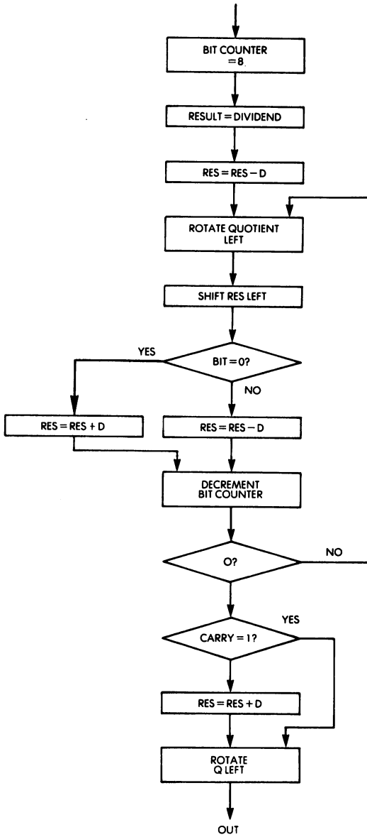
Fig. 3-20: 16 by 8 Division Flowchart
