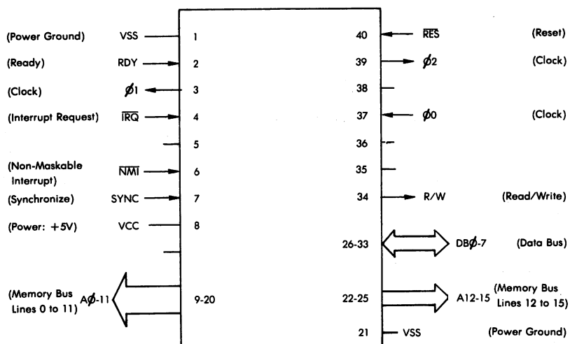
Fig. 2-7: 6502 Pinout
