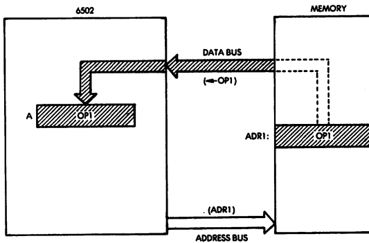
Fig. 3-2: LDA ADR1: OP1 is Loaded from Memory
