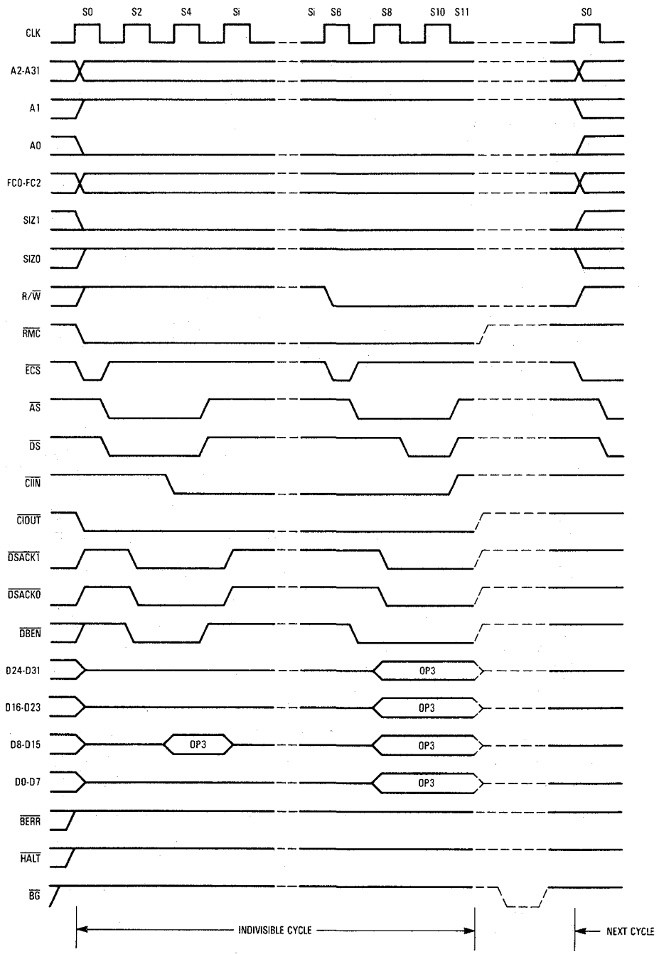
Figure 7-30. Asynchronous Byte Read-Modify-Write Cycle — 32-Bit Port (TAS Instruction with \overline{CIOUT} or \overline{CIIN} Asserted)
