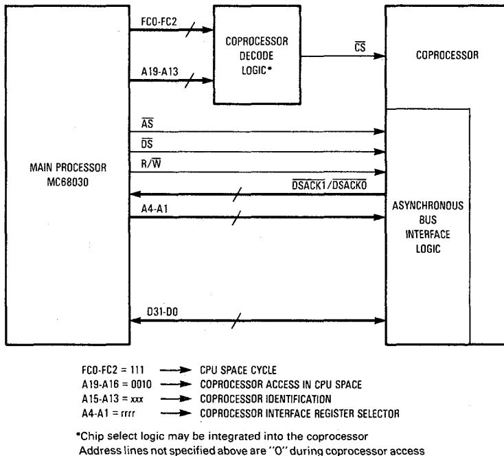
Figure 10-2. Asynchronous Non-DMA M68000 Coprocessor Interface Signal Usage
