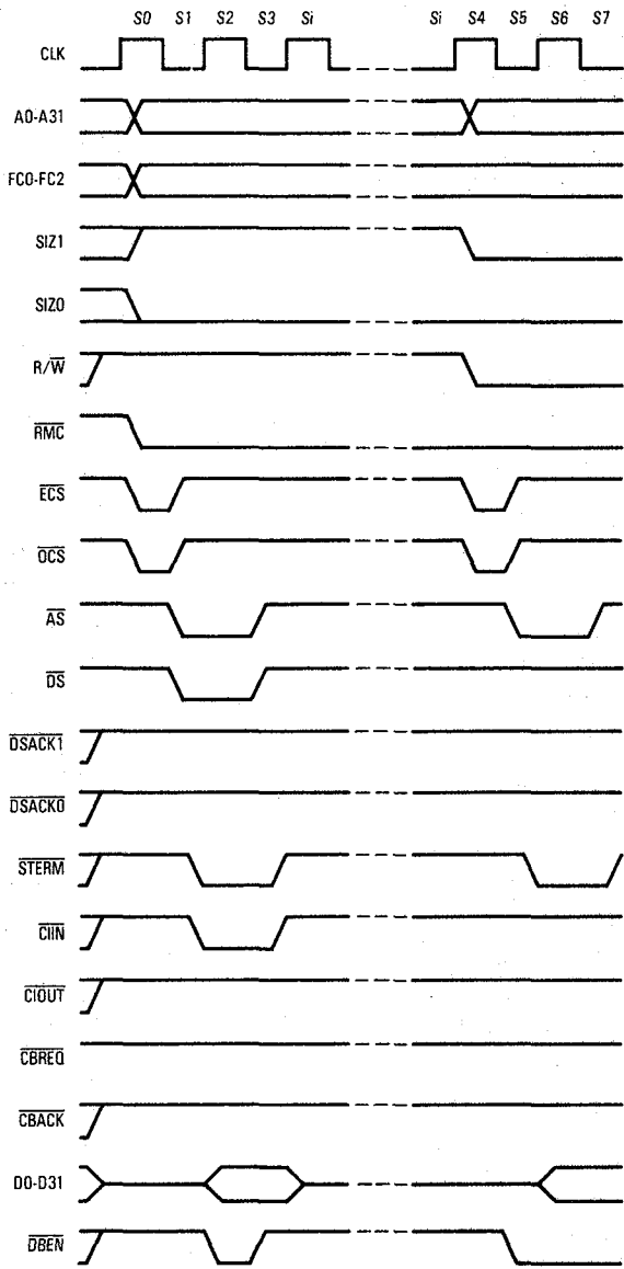
Figure 7-36. Synchronous Read-Modify-Write Cycle Timing — \overline{\text{CIIN}} Asserted
