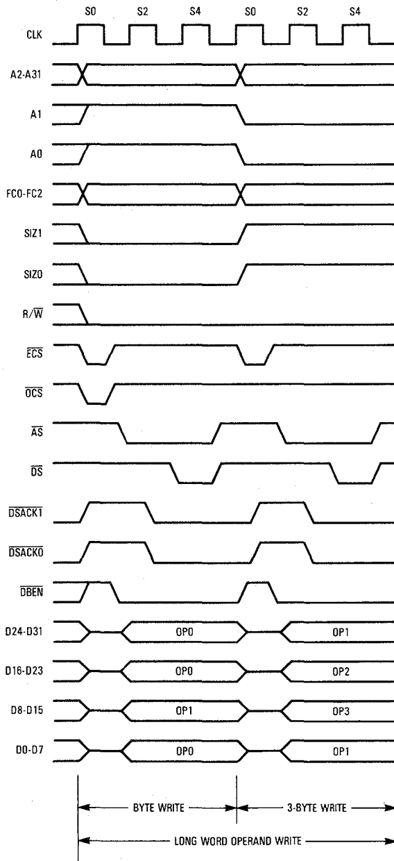
Figure 7-16. Misaligned Write Cycles to Long-Word Port
