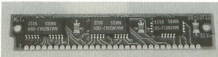
Figure 6-6 Some manufacturers use a combination of PLCC and SOJ DRAM chips.
