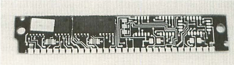
Figure 6-5 SOJ SIMM PCB layouts vary from manufacturer to manufacturer.
