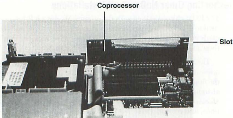
Figure 7-13 Optional adapter cards for the Macintosh IIsi include an MC68882RC20A math coprocessor and either a NuBus expansion slot or an MC68030 processor-direct expansion slot.
