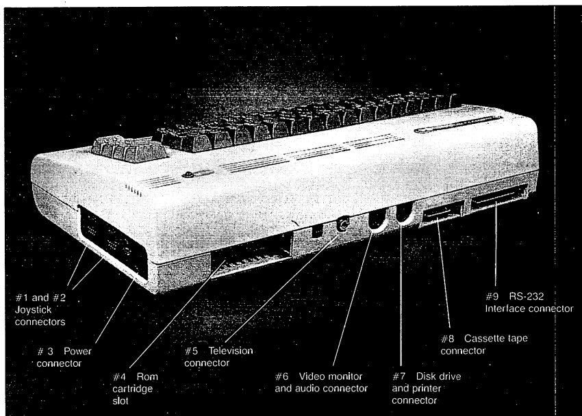
FIGURE A.1 Connectors on the Commodore 64
