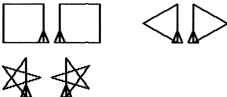
Figura 5.21 Figure speculari
