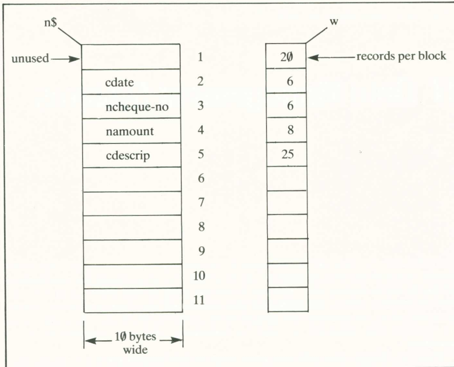
Figure 17.1 Header block layout.
