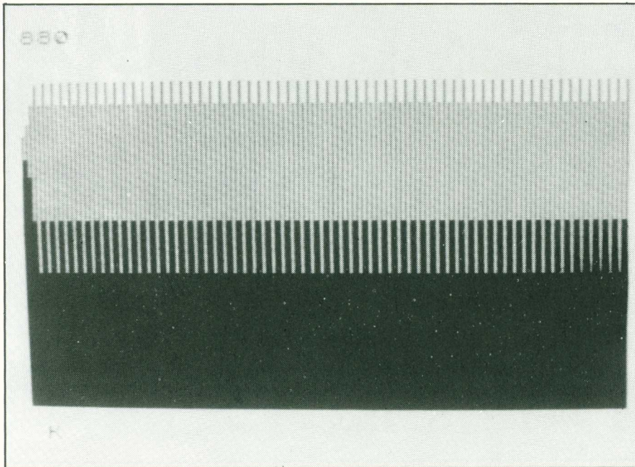
Figure 5.2 Graphic display: k = 880 . Period 4.
