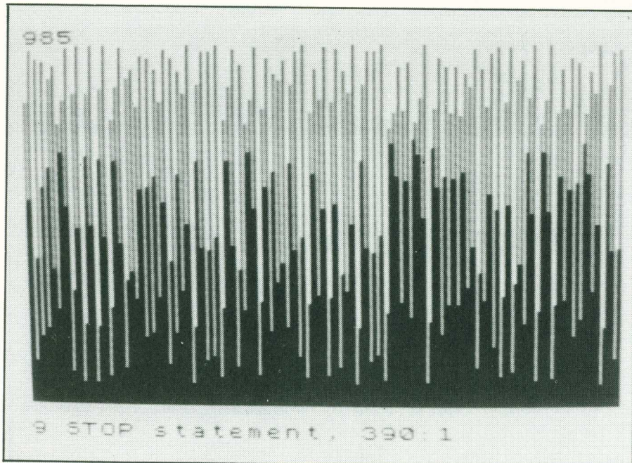
Figure 5.4 Graphic display: k = 985 . Chaos!
