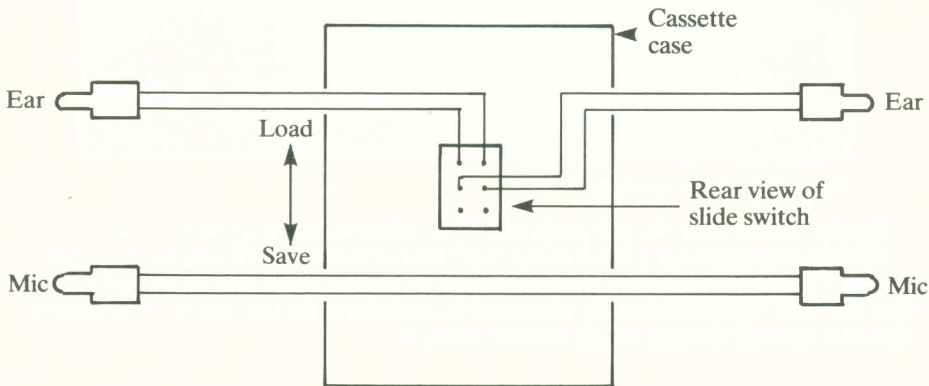
Figure E.1 Circuit diagram for LOAD/SAVE switch.
