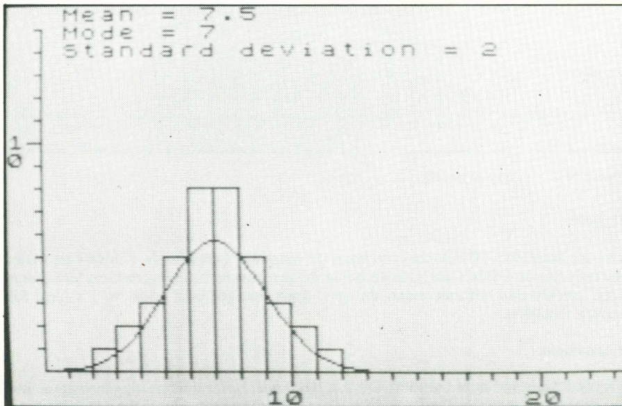
Figure 10.3 Normal curve approximating a histogram fairly well . . .
