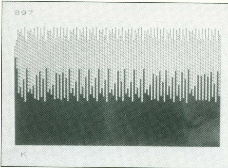
Figure 5.3 Graphic display: k = 897 . Traces of periodicity remain.
