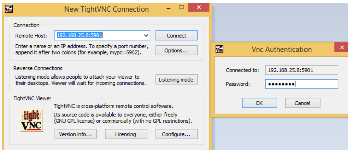
Figura 4.2: TightVNC
