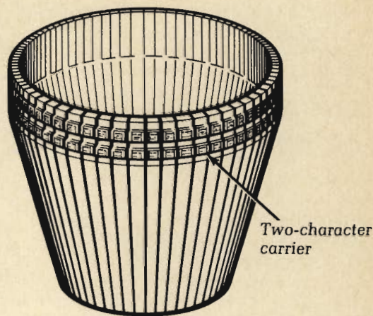
Another kind of printing element is the thimble, which looks like a daisy wheel with the spokes bent up.
