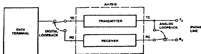
Figure 3. Loopback Configurations
