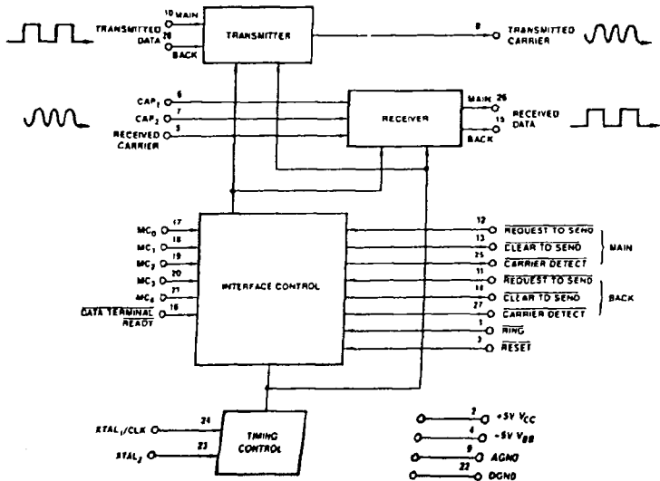
Figure 2. Am7910 Block Diagram
