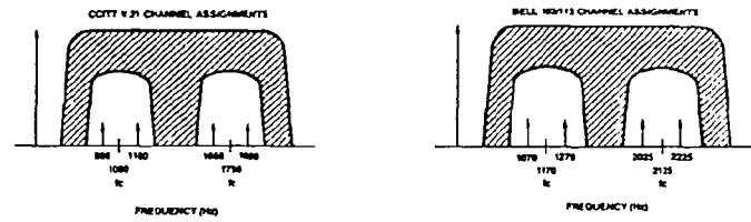
Figure 6. Full Duplex
