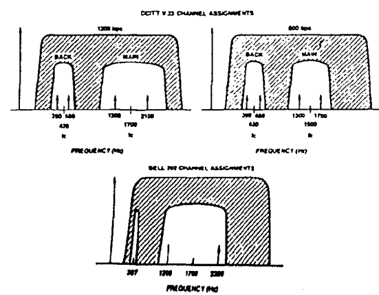
Figure 7. Half Duplex
