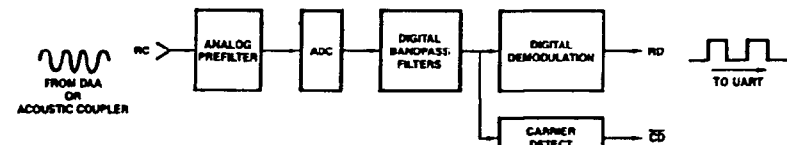
Figure 5. Receiver Block Diagram
