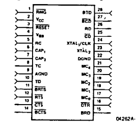
Figure 1. Connection Diagram
