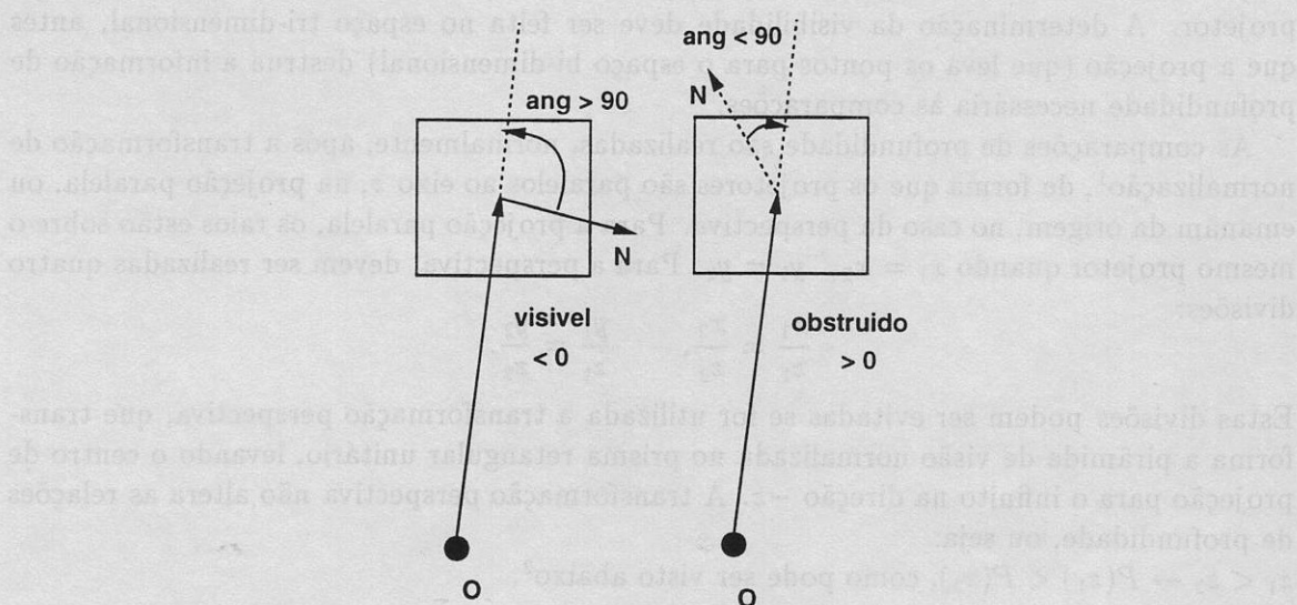
Figura 11.2: Back-Face Culling.
