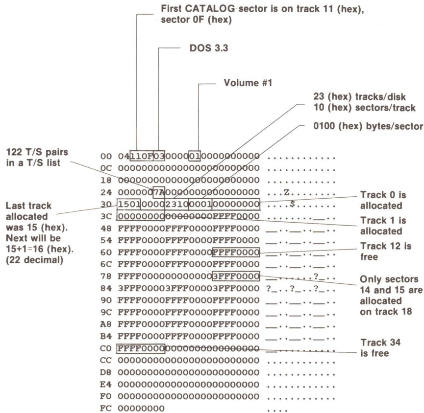
FIGURE 4.2 — EXAMPLE VTOC
