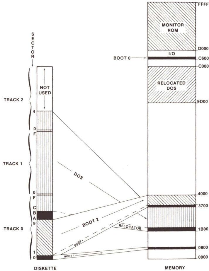
FIGURE 5.2 - BOOTSTRAP PROCESS
