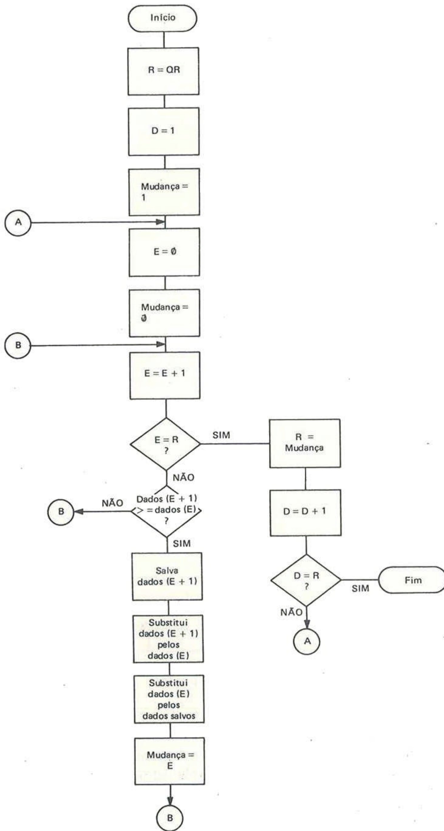
Figura 10 Bubble-Sort.
