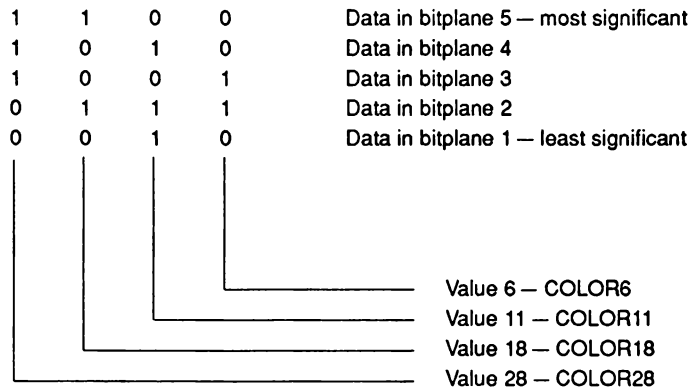
Figure 3-4: Significance of Bitplane Data in Selecting Colors
