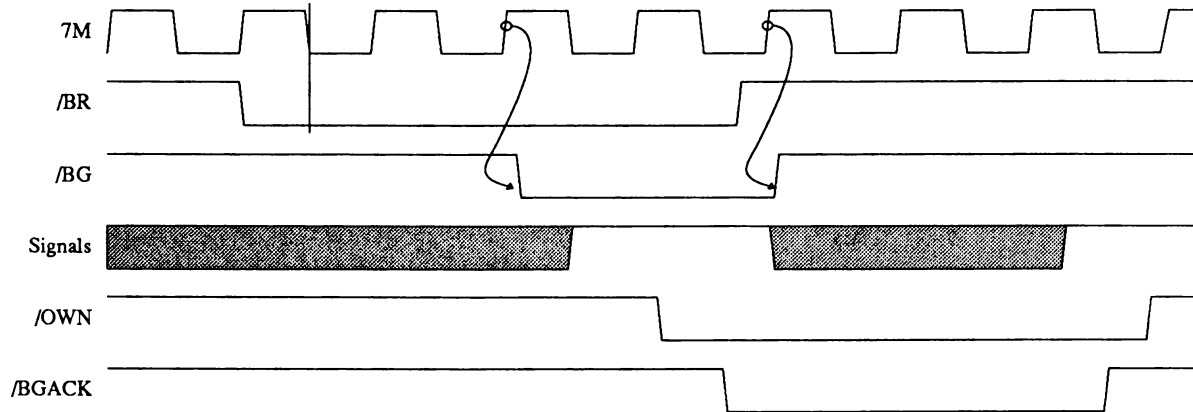
Figure K-4: Zorro II Bus Arbitration
