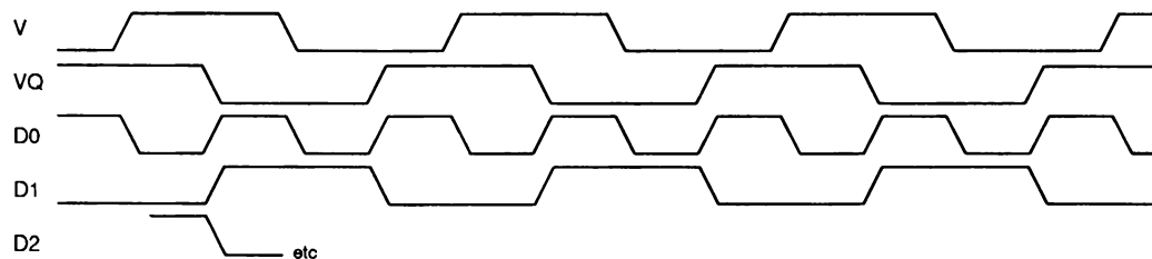
Figure 8-2: Mouse Quadrature
