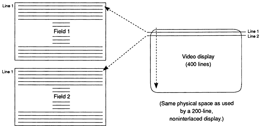
Figure 3-5: Interlacing
