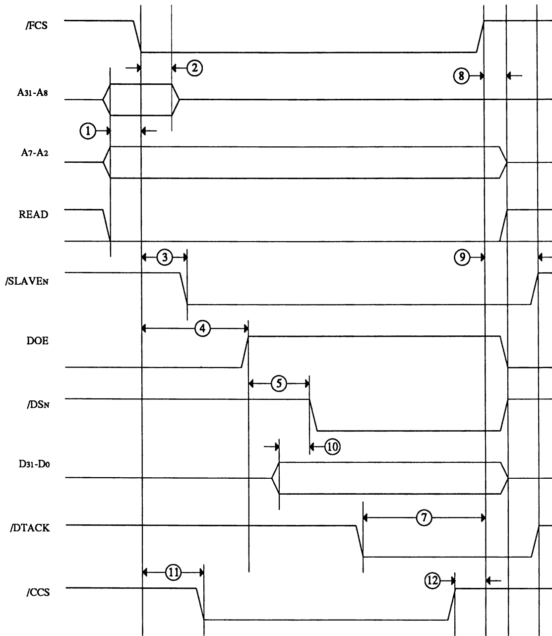
Figure K-11: Write Cycle Timing
