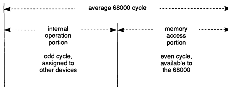
Figure 6-10: Normal 68000 Cycle
