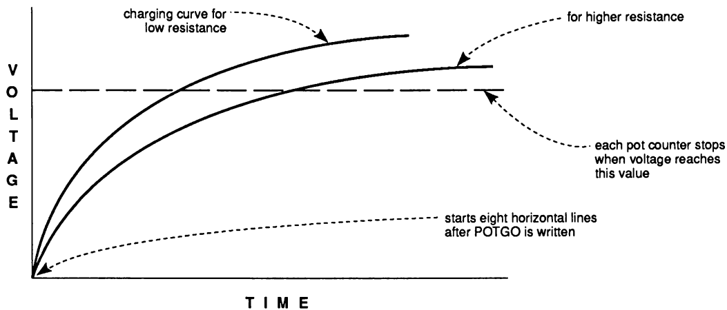
Figure 8-5: Effects of Resistance on Charging Rate
