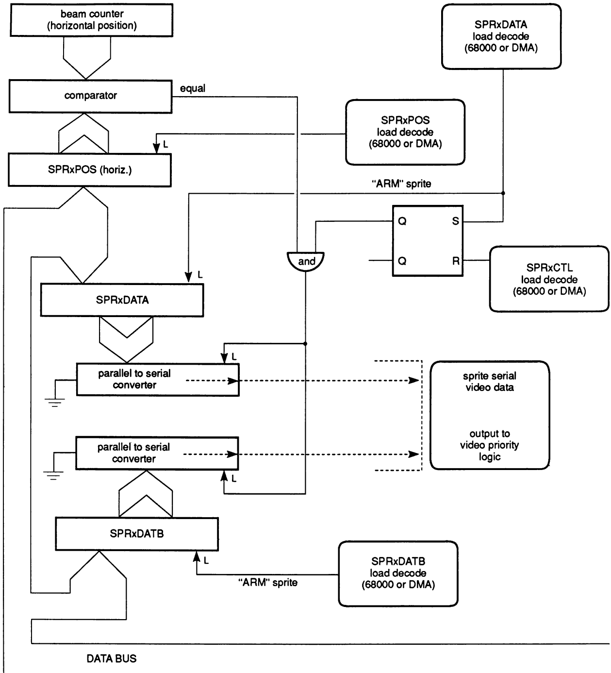
Figure 4-13: Sprite Control Circuitry
