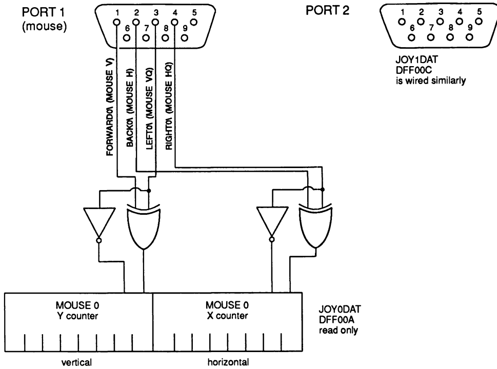
Figure 8-3: Joystick to Counter Connections
