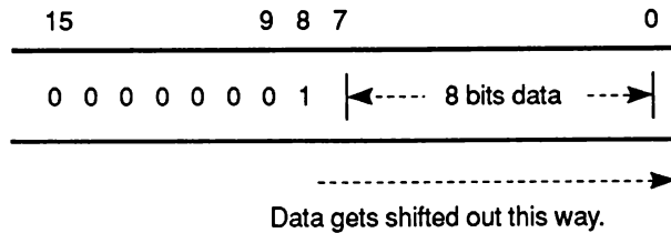
Figure 8-12: Ending Appearance of Shift Register
