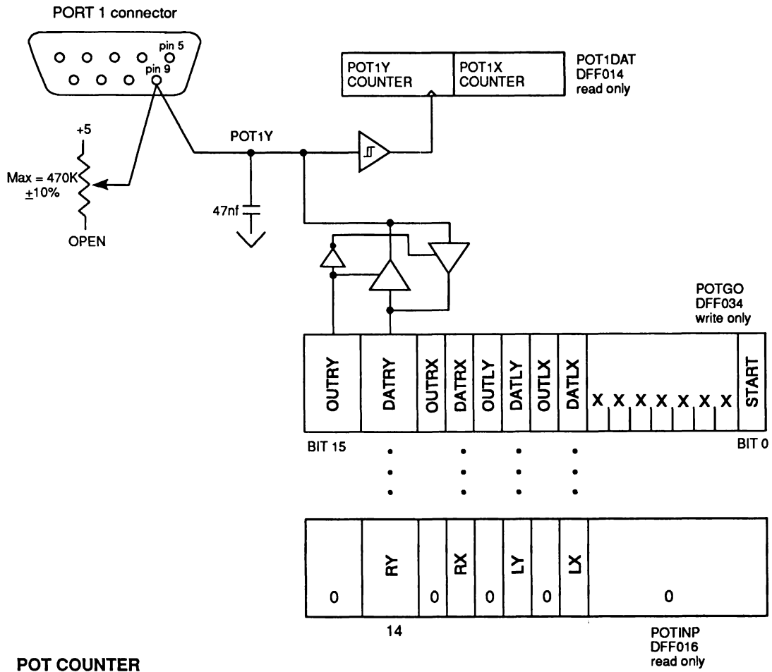
Figure 8-6: Potentiometer Charging Circuit
