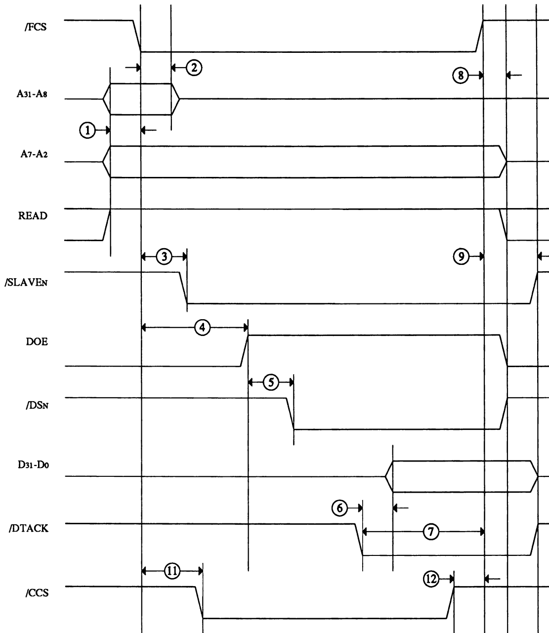
Figure K-10: Read Cycle Timing
