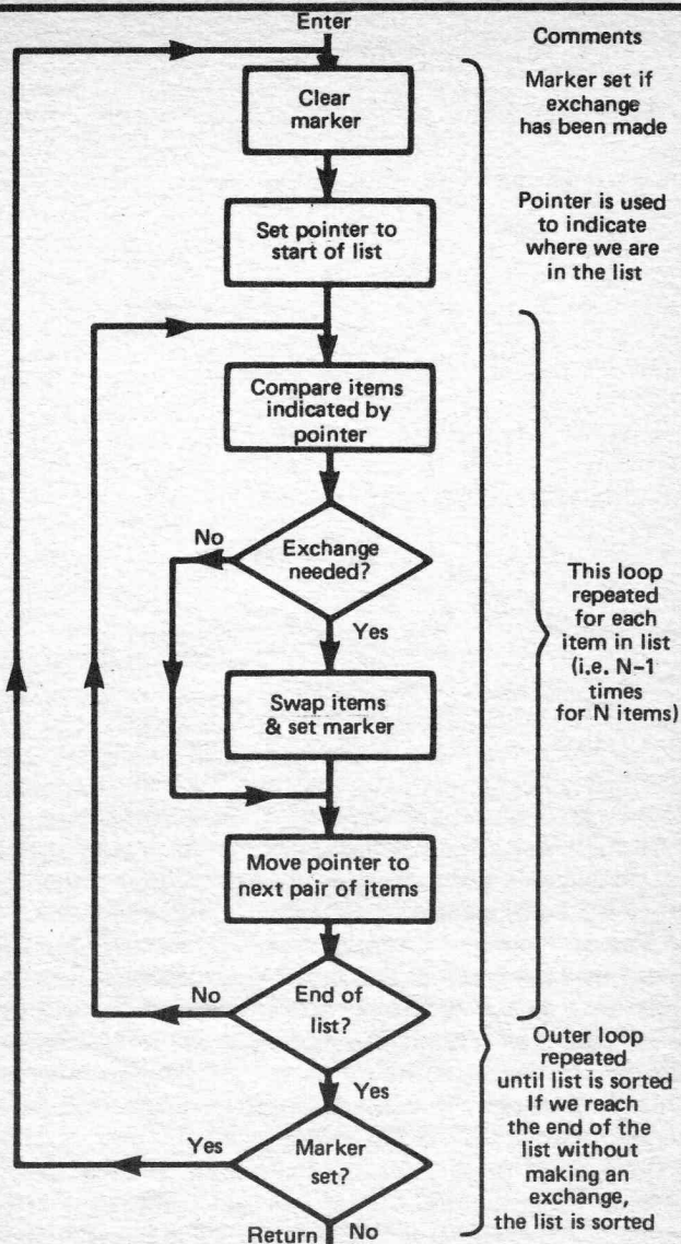
Fig. 5.1 Flowchart for bubble sort
