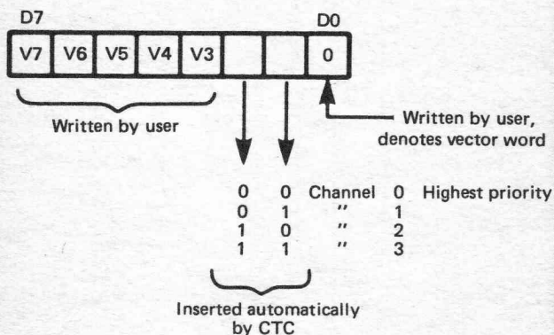
Fig. 6.24 CTC interrupt vector
