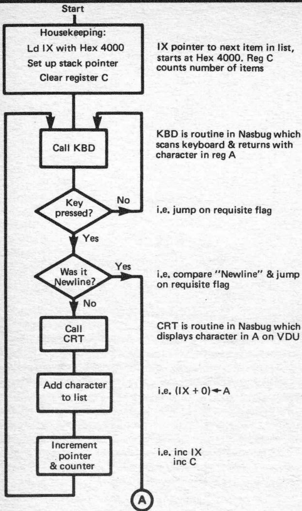
Fig. 5.4 (a) Detailed flow chart for bubble sort test program
