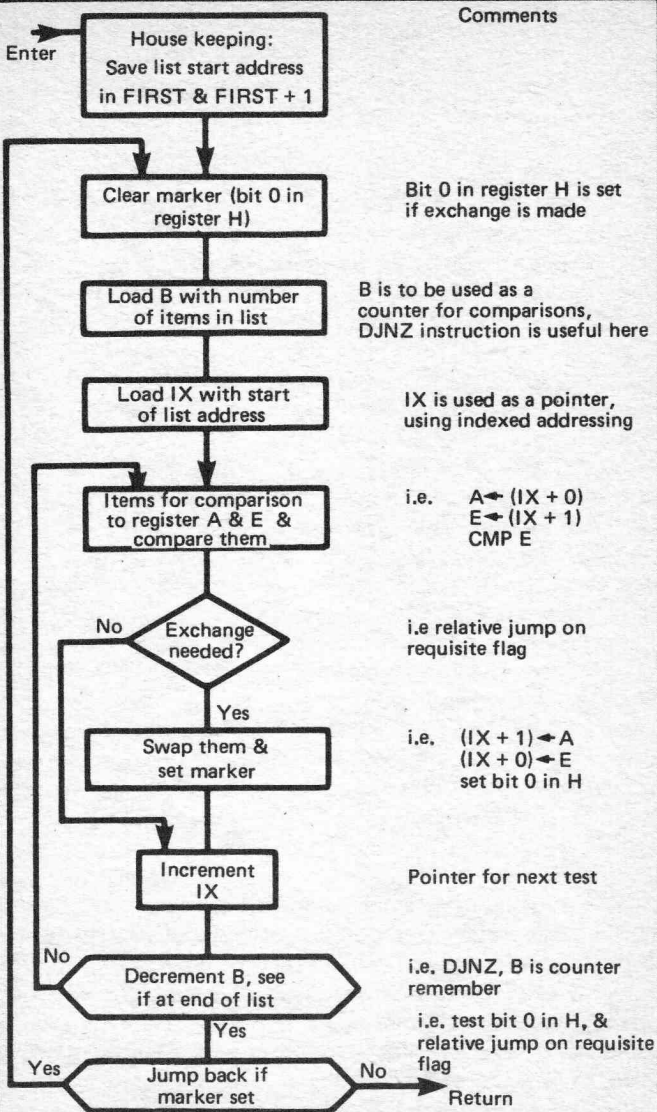
Fig. 5.2 Detailed bubble sort flow chart
