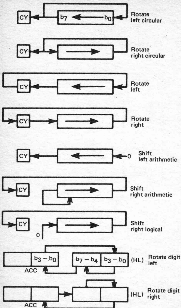
Fig. 4.2 Z-80 rotate & shift instructions
