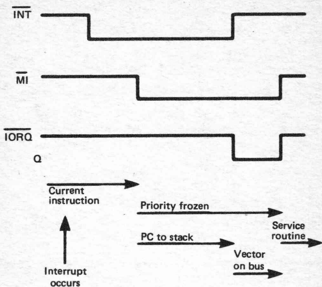
Fig. 6.7 Simplified interrupt timing
