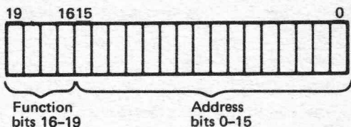
Fig. 3.1 Instruction on a minicomputer
