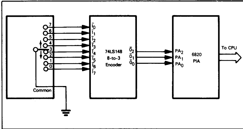
Figure 11-12. A Multiple-Position Switch with an Encoder
