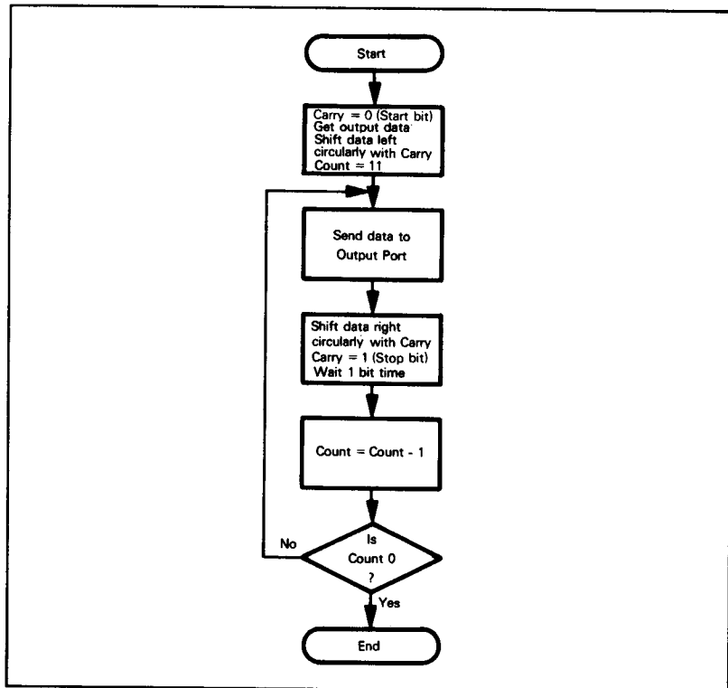
Figure 11-28. Flowchart for Transmit Procedure
