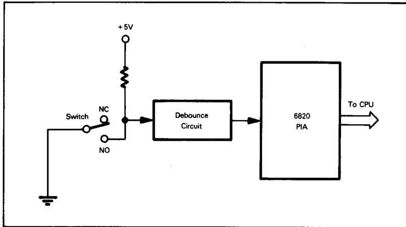
Figure 11-9. A Toggle Switch Circuit
