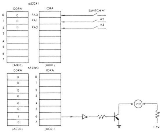
Fig. 5-40: The Connections
