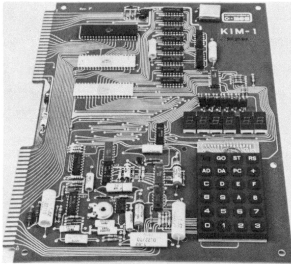
Fig. 3-2: Photo of KIM-1
