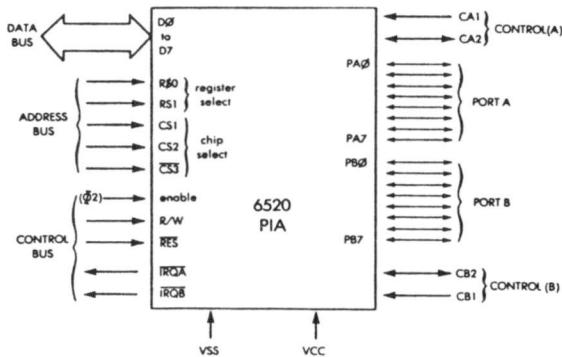
Fig 2-2: The 6520 PIA
