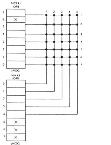
Fig. 5-16: Connecting the 5x7 LED
