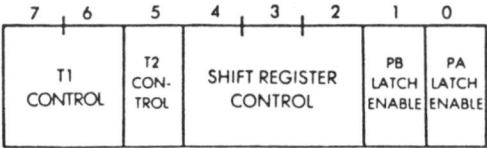
Fig. 2-27: 6522 - Auxiliary Control Register
