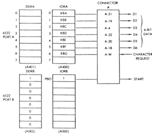
Fig. 6-19: Printer Connection
