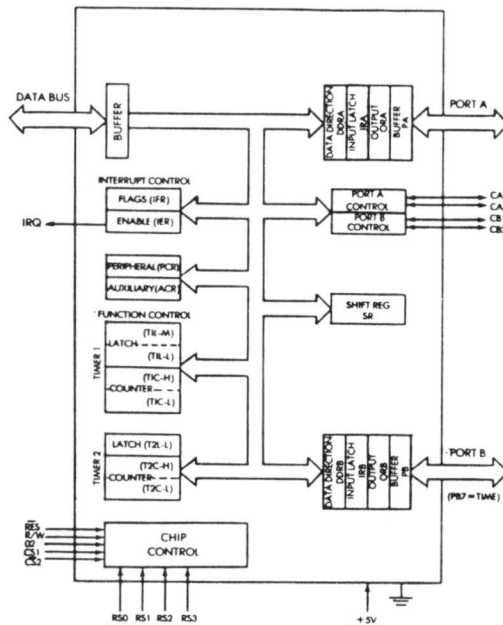
Fig 2-14: 6522 Internal Architecture
