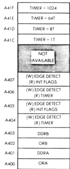
Fig. 3-15: Memory Map for the 6532
