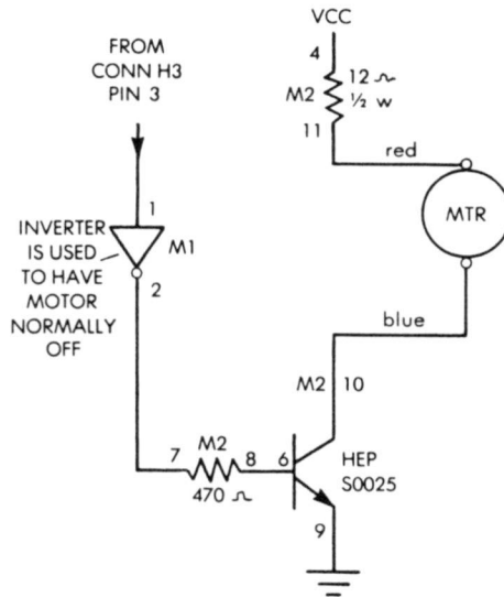
Fig. 5-36: Motor Circuit
