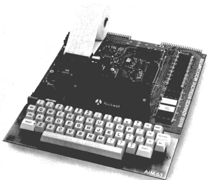
Fig 3-18 : AIM 65 is a Board with Mini-Printer and Full Keyboard
