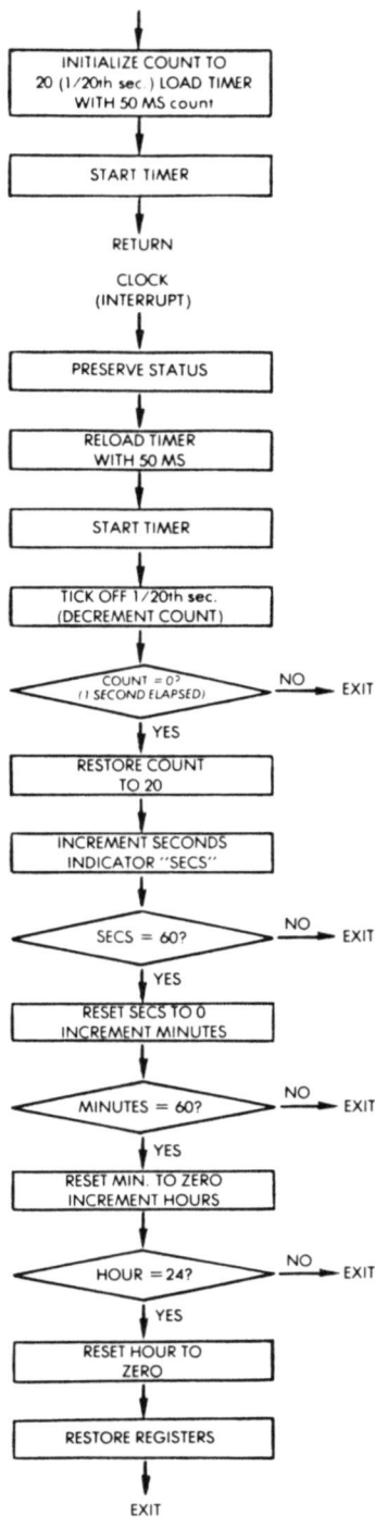
Fig. 4-36: Time-of-Day Clock
