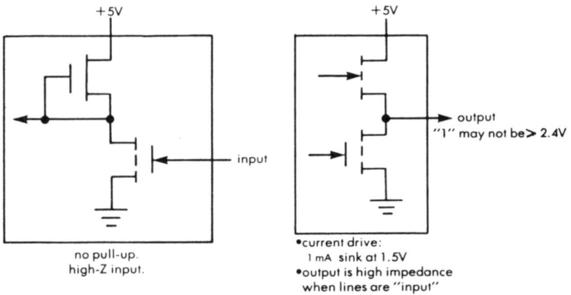
Fig. 2-5: Buffer B
