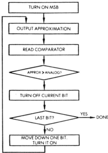
Fig. 5-46: Successive Approximation Flow Chart
