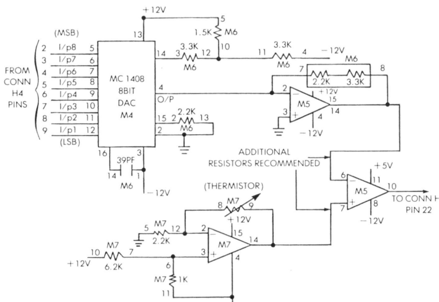
Fig. 5-47: ADC Interface
