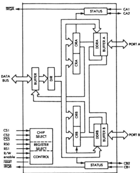
Fig 2-3: 6520 Internal Architecture
