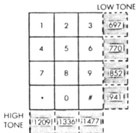
Fig. 4-39: The Telephone Frequencies
